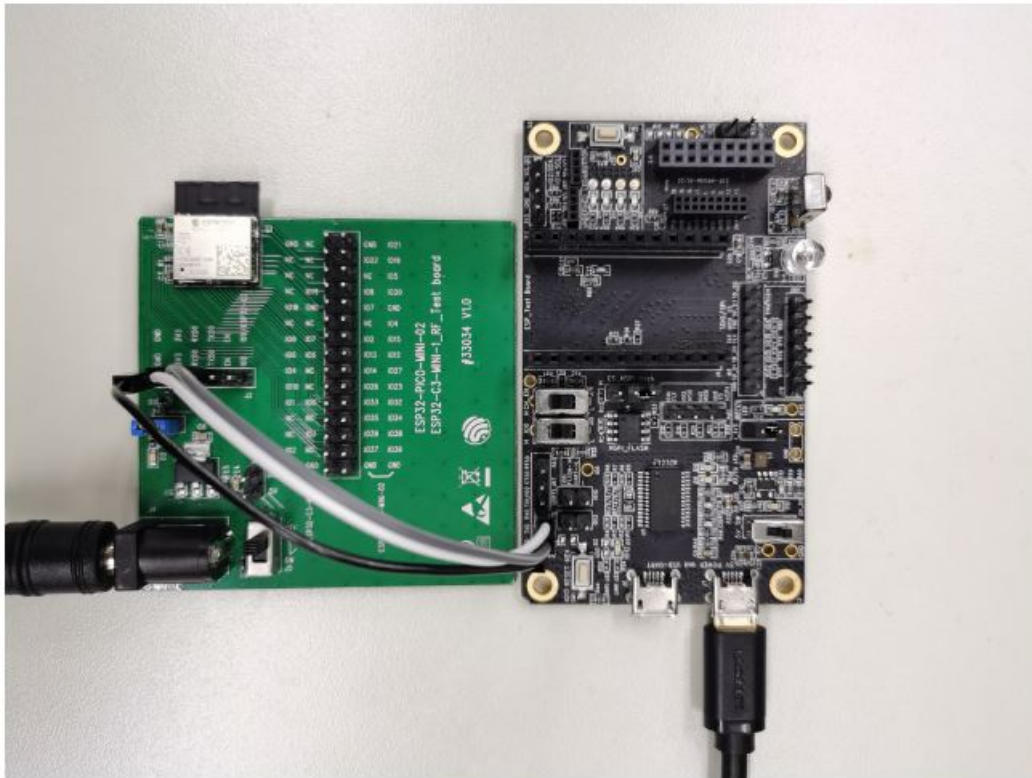
Figure 2: Hardware Connection
