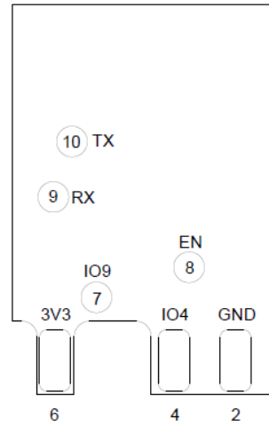
Pin Layout (Bottom View)
