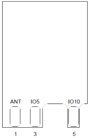
Pin Layout (Top View)
