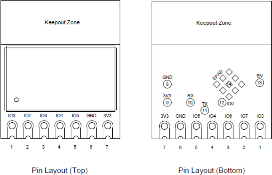
Figure 1: Pin Layout (Top View)
