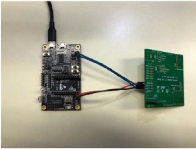
Figure 2: Hardware Connection
