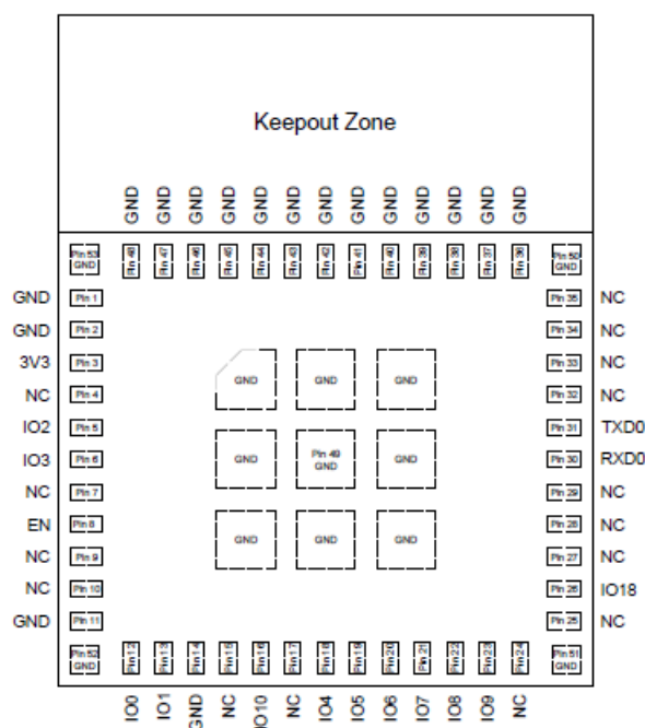
Figure 1: Pin Layout (Top View)
