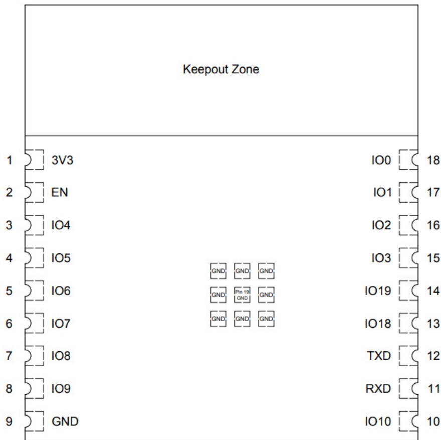
Figure 1: Pin Layout (Top View)
