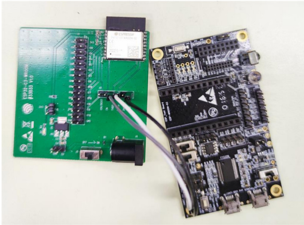
Figure 2: Hardware Connection
