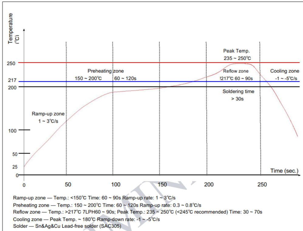
Figure 2: Reflow Profile
