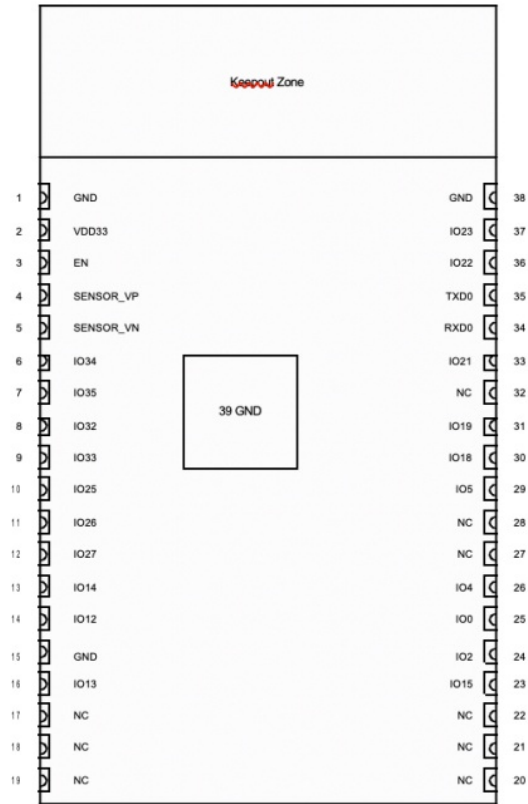
Figure 1: Pin Layout of ESP32-WROVER-E (Top View)
