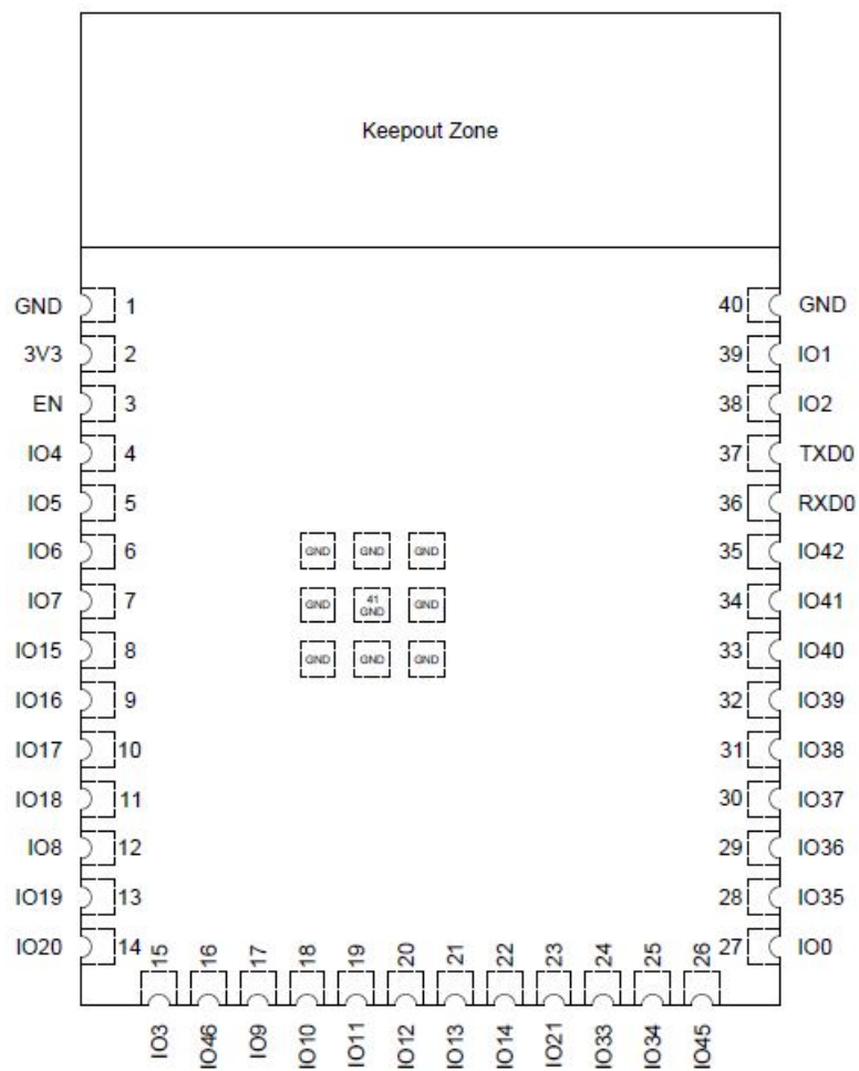
Figure 1: Pin Layout (Top View)
