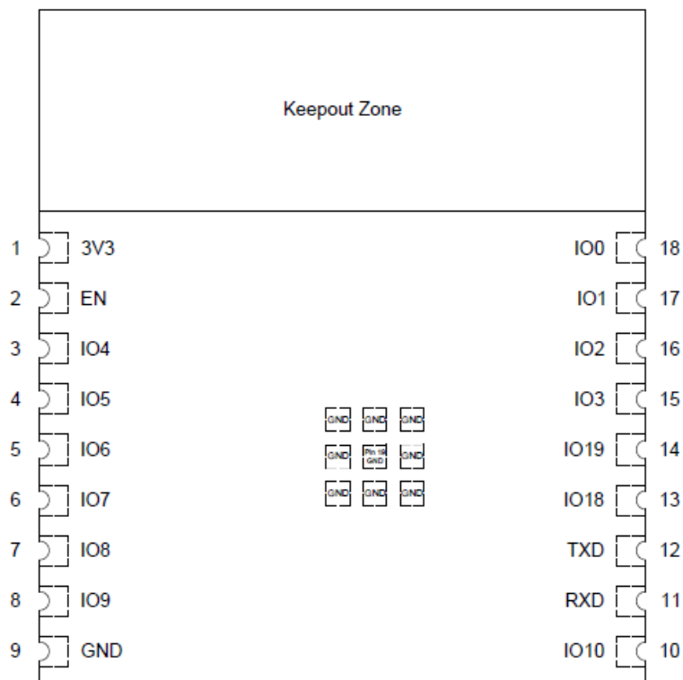
Figure 1: Pin Layout (Top View)
