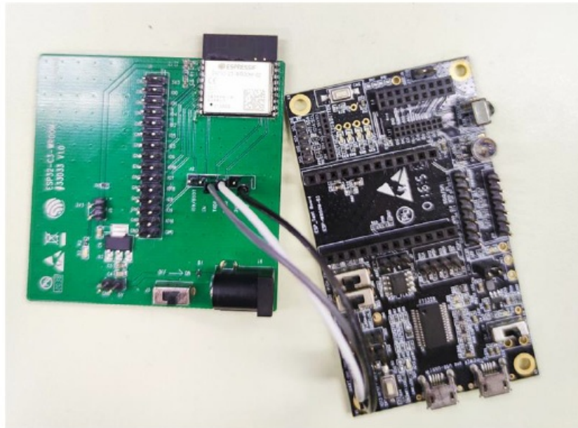
Figure 2: Hardware Connection
