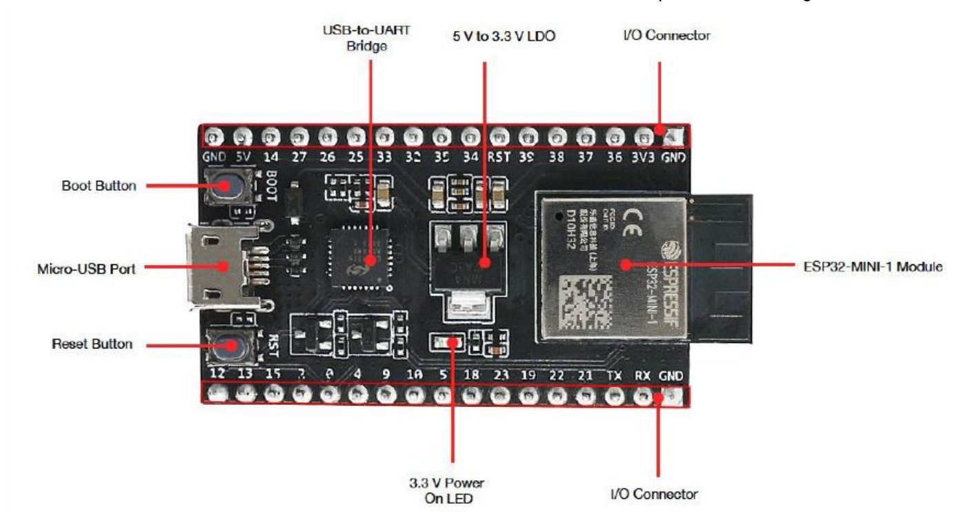
ESP32-DevKitM-1 – front
