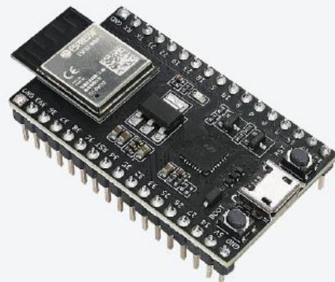
ESP32-DevKitM-1 - isometric
