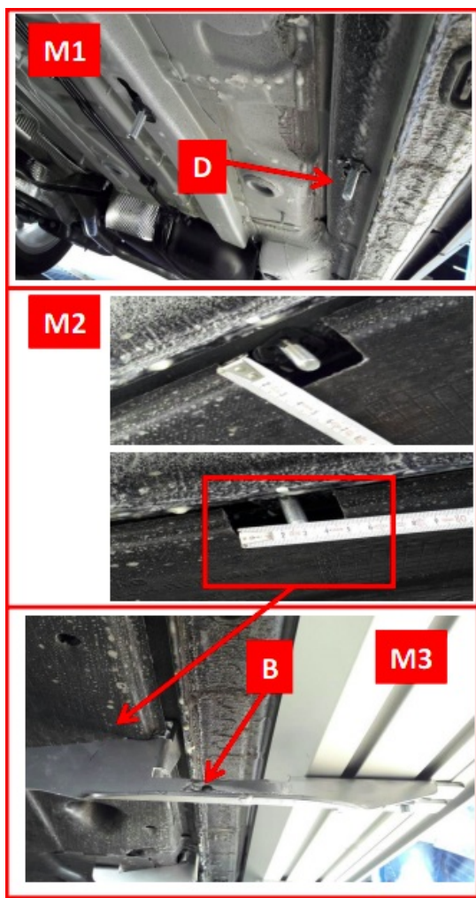
REAR BRACKET
