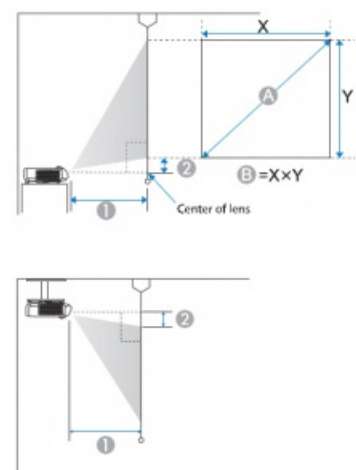
Projection Distance Table (EB-535W/525W)
