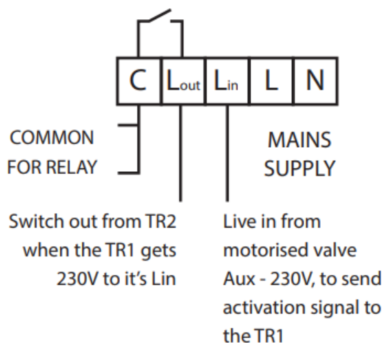
Internal wiring diagram TR2
