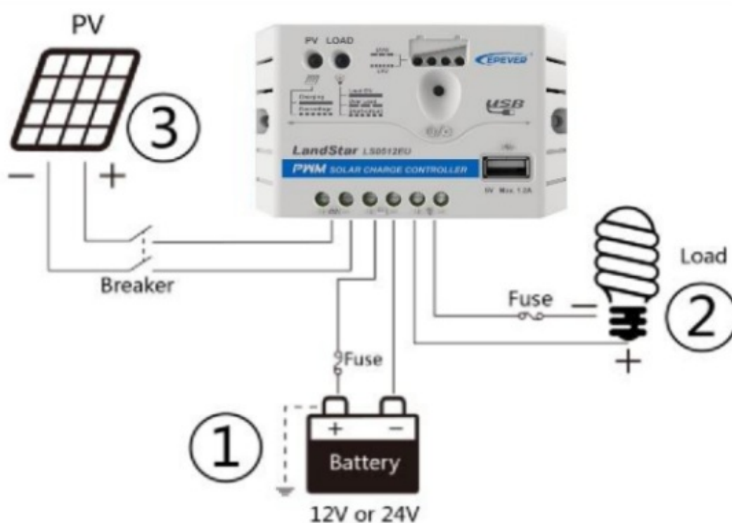
Figure 2 Connection diagram
