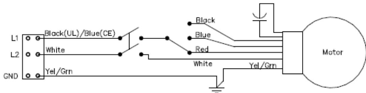
Figure 10: Wiring Diagram 3-Speed
