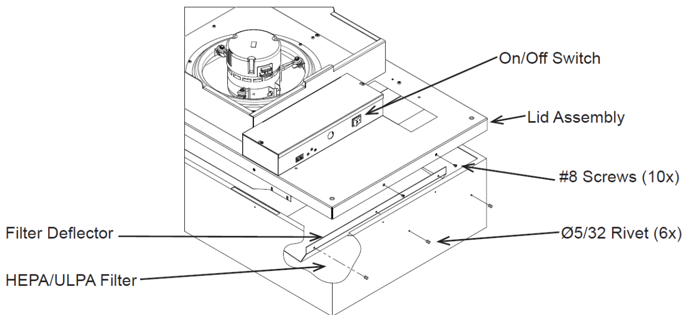
Figure 5: Standard Filter Change
