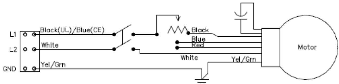
Figure 11: Wiring Diagram Speed Control
