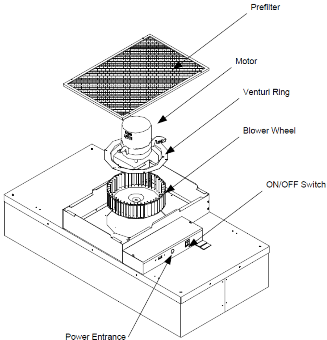
Figure 8: Standard/RSR Motor Replacement
