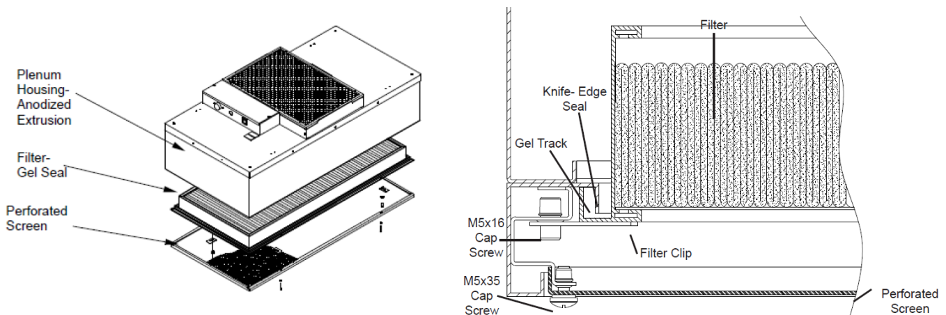
Figure 6: RSR Extrusion Filter Replacement
