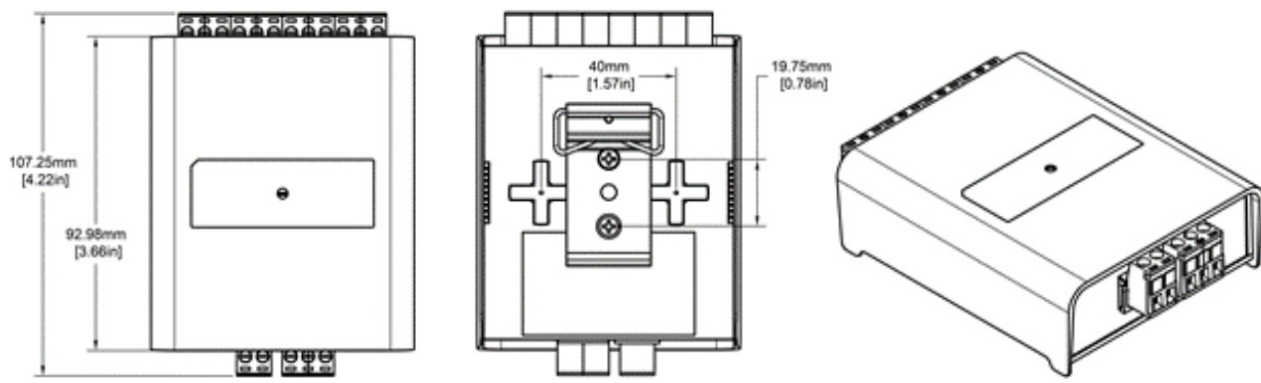
BOTTOM VIEW
