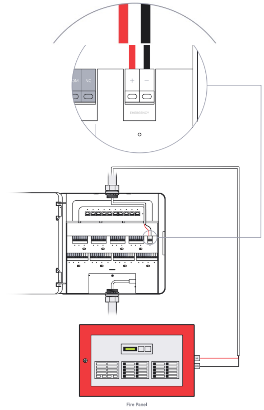
Fire Panel
