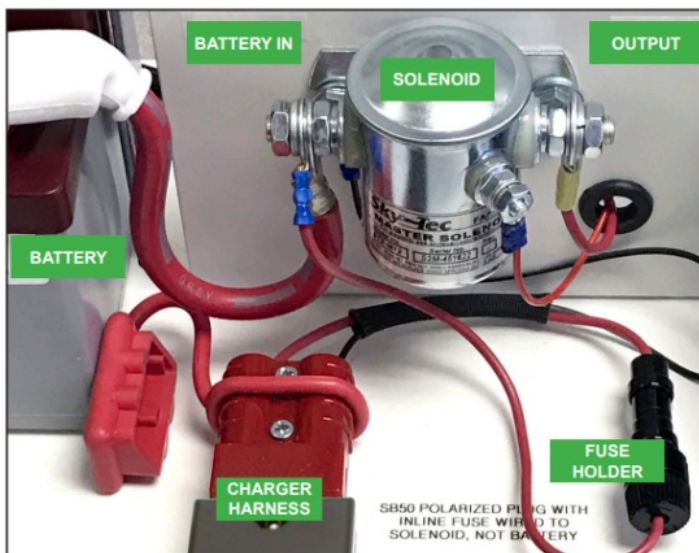
Figure 1. Simplified example of connection to battery solenoid. For more examples, see www.audioauthority.com/BM-AIK .
