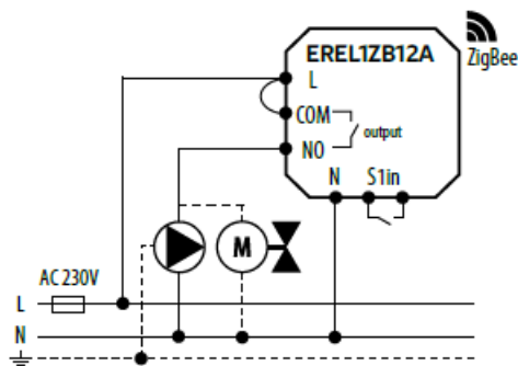
3. c) Connection diagram for pump / actuator
