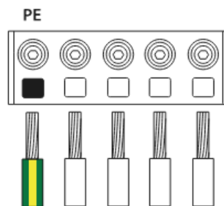
TN 3-phase (230 V)
