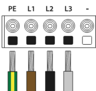
IT/TT 3-phase (230 V)
