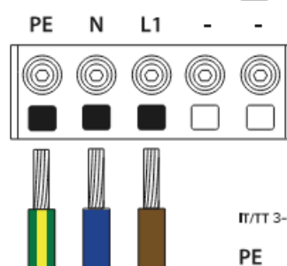
TN 1-phase (230 V)
