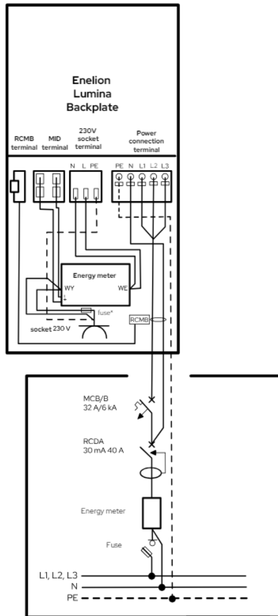
Power connection in the case of measuring the entire ENELION LUMINA charger.
