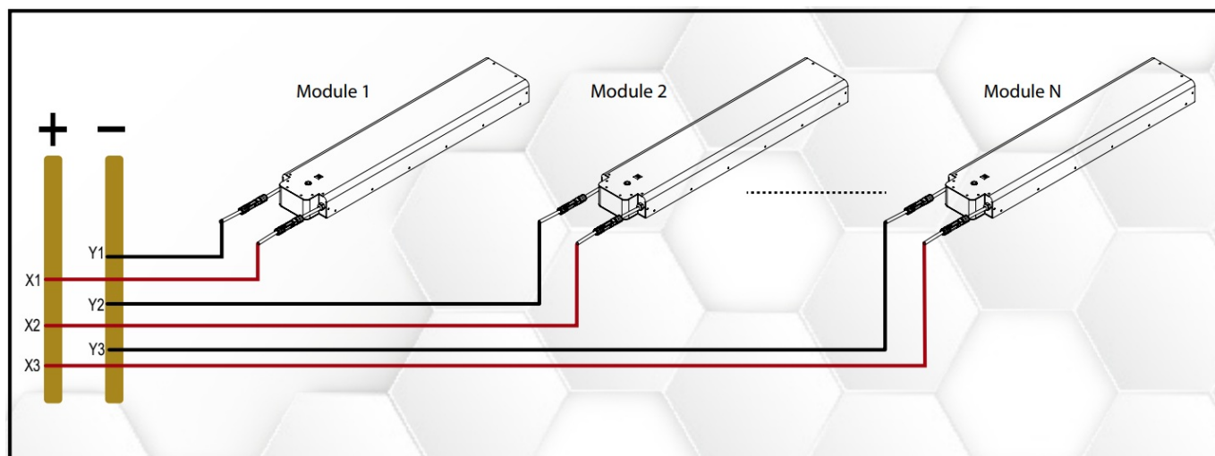
Figure 6: Modules connected in parallel
