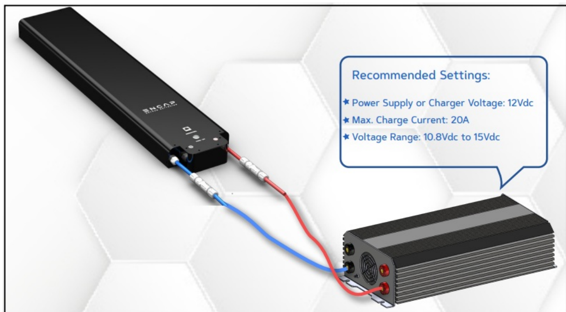
Figure 4: Charging Module with power supply
