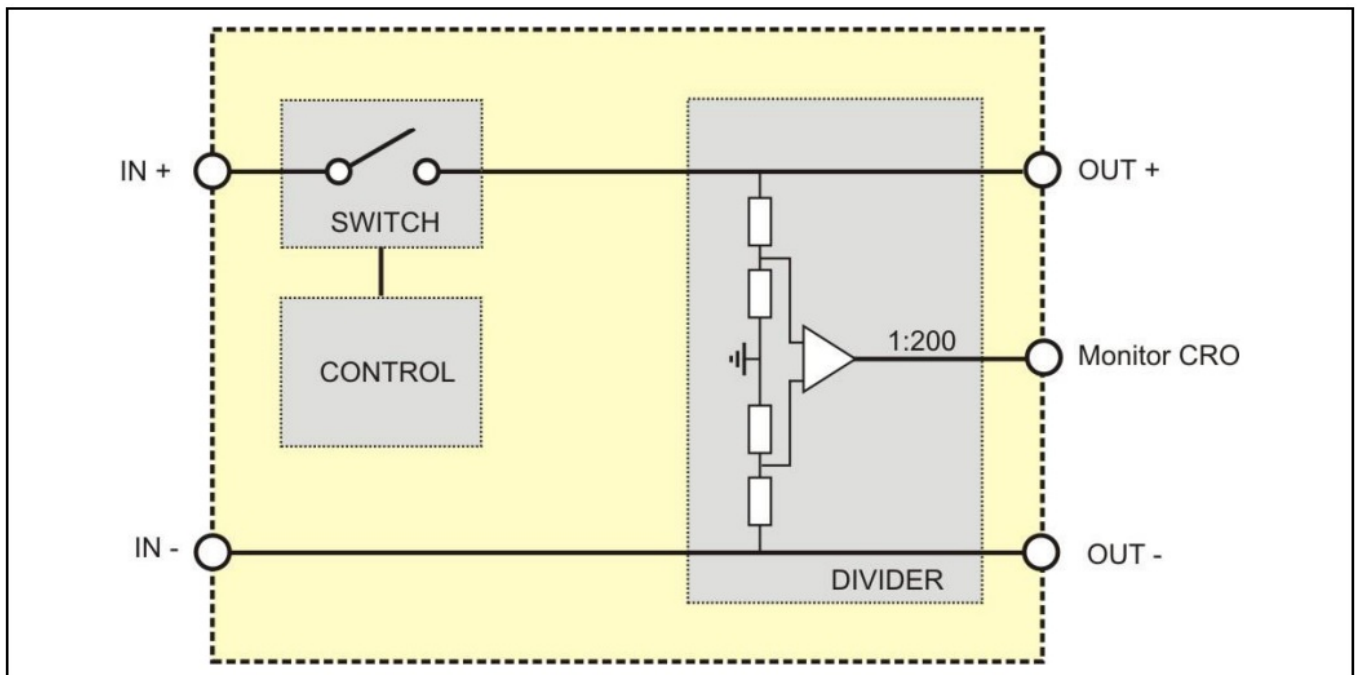
Figure 9.1.: Overview BS 200N100
