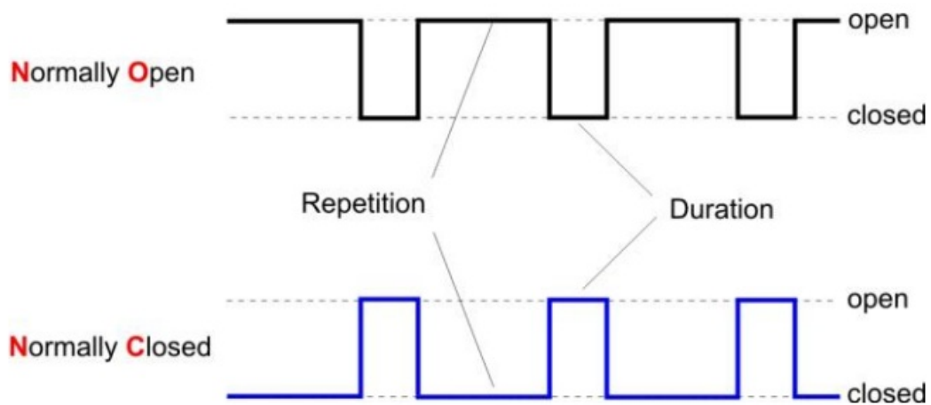
Figure 3.2. : Operating modes Switch BS 200N100
