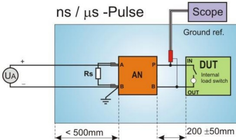
Figure 7.3: Setup for DUT with internal switch for \mu\text{s} / ns pulses
