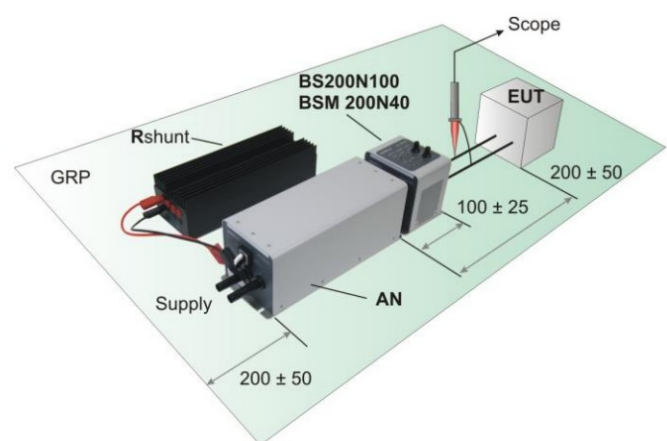
Figure 7.2.: Setup for pulses in the \mu s / ns range
