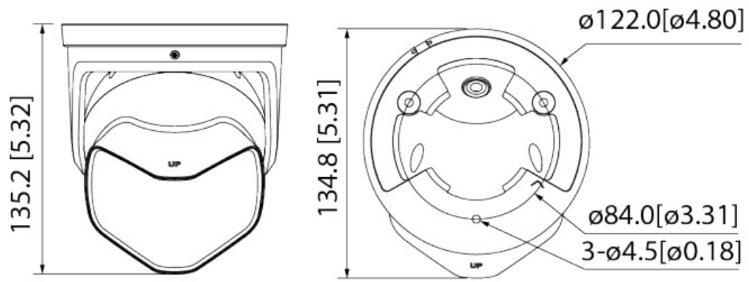
Figure 3-4 Dimensions: Model C (mm [inch])
