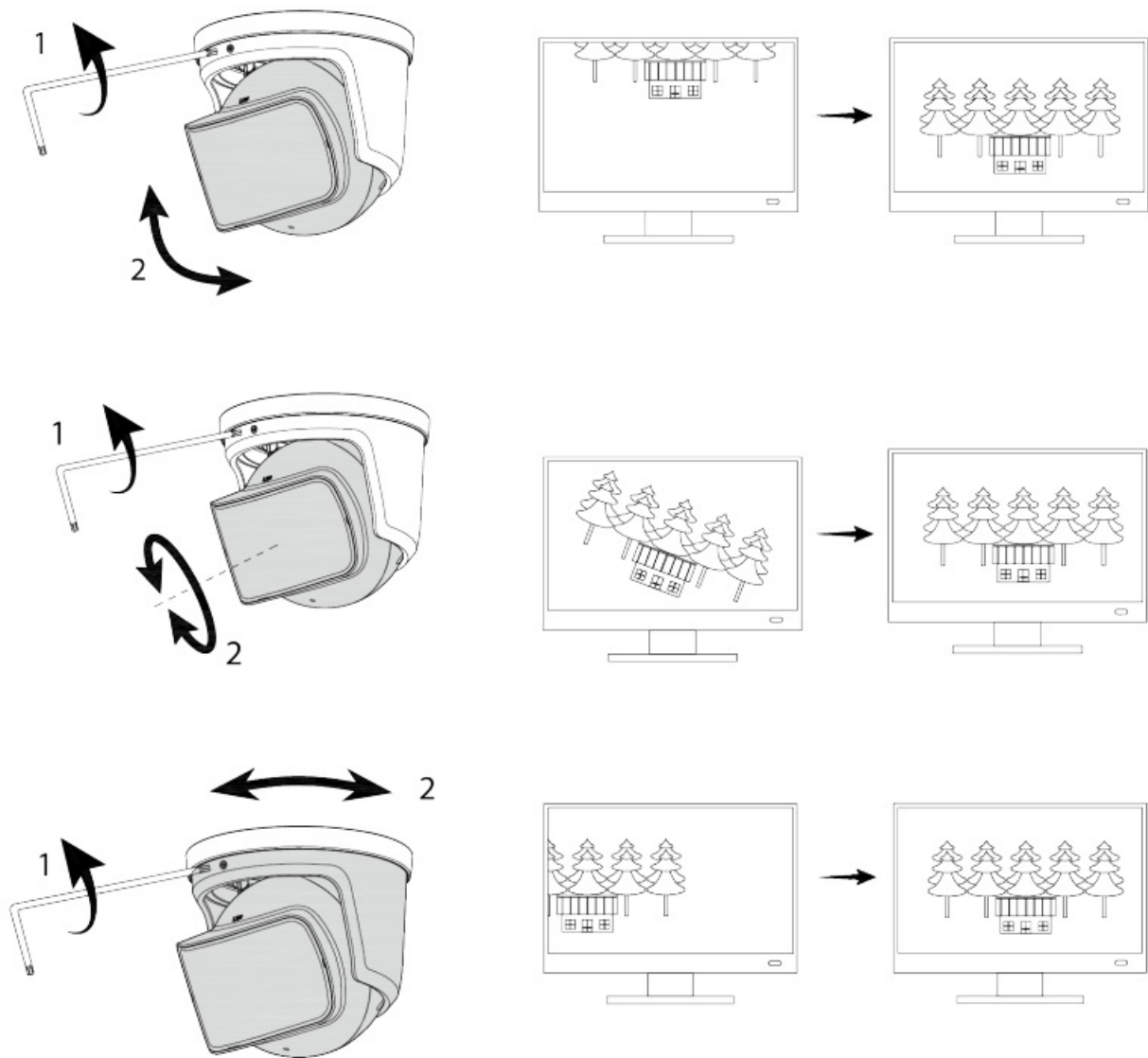
Figure 3-10 Adjust lens angle
