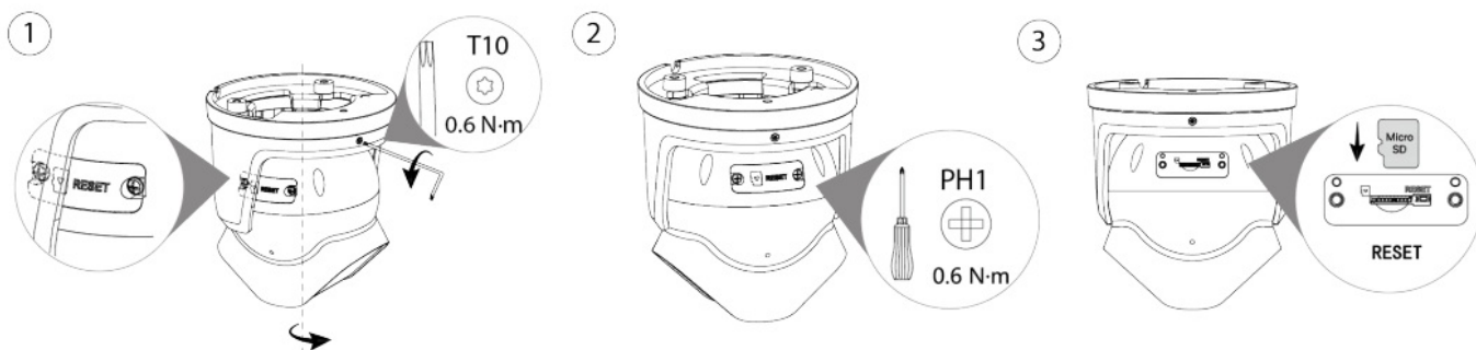
Figure 3-6 Install the SD card
