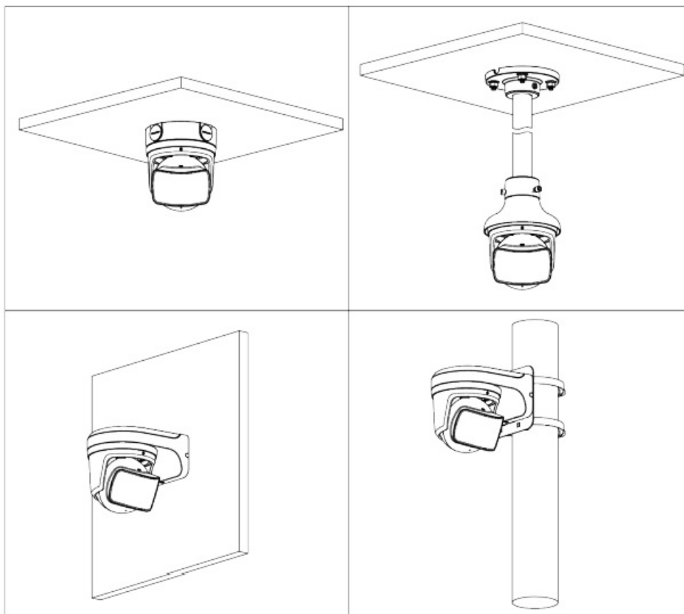
Figure 3-5 Installation methods
