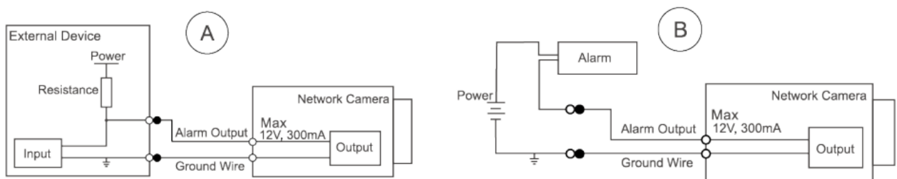
Figure 1-4 Alarm output
