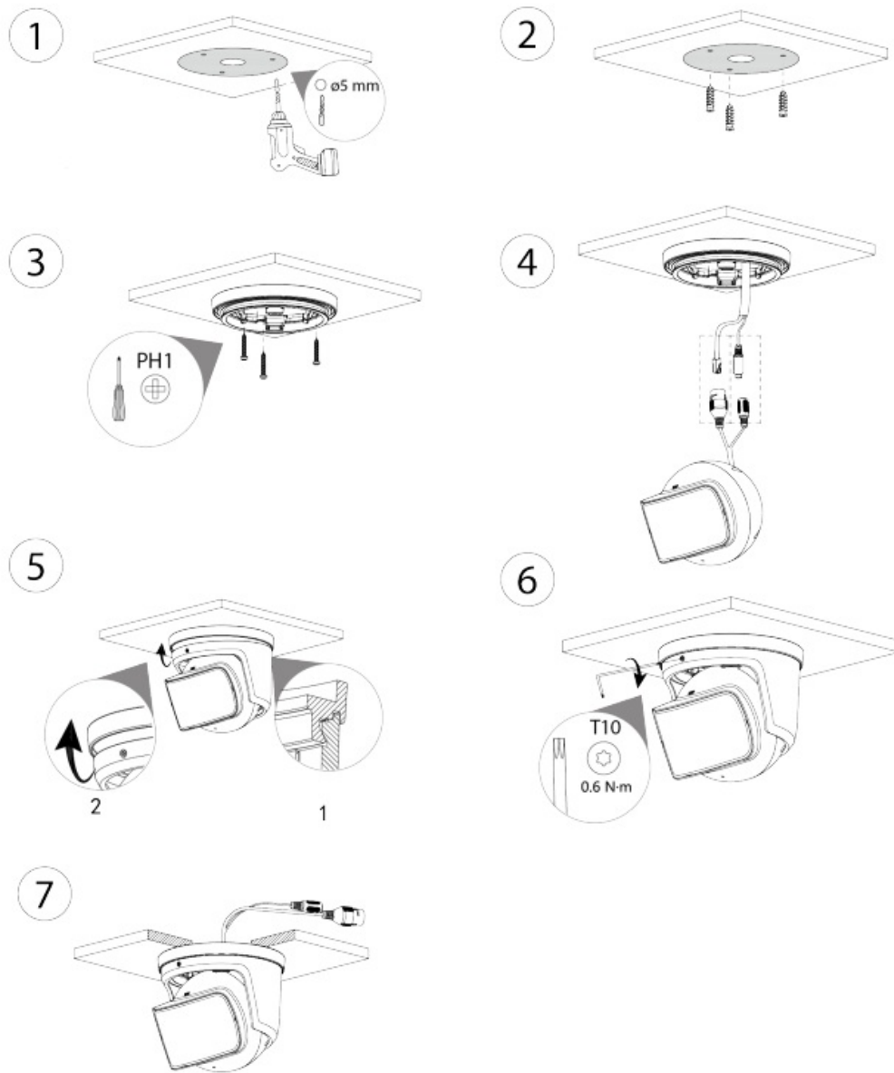
Figure 3-8 Cable going through the mounting surface
