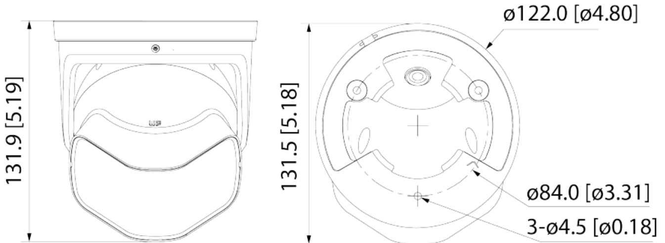
Figure 3-2 Dimensions: Model A (mm [inch])
