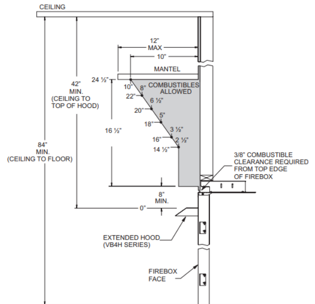
Figure 3b - Mantel Clearances with Optional Extended Hood
