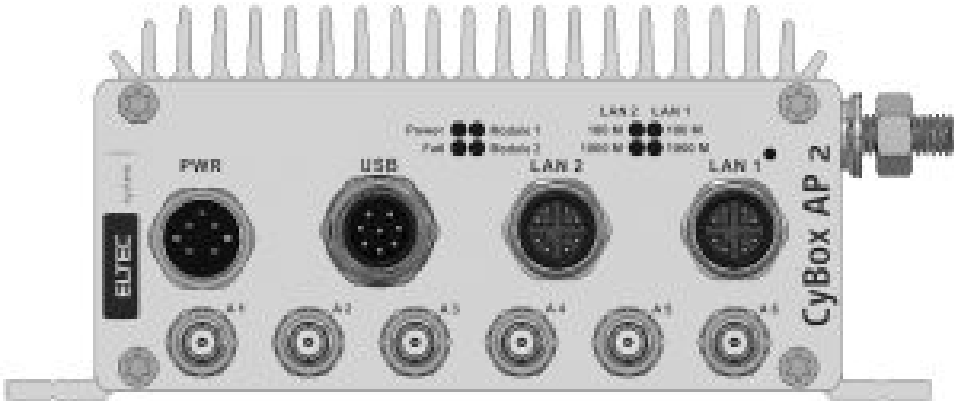
Figure: 3 Front Panel Overview
