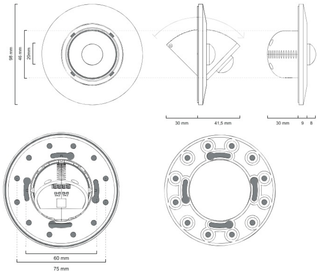
Dimensions of mounting ring
