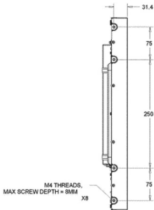
SIDE MOUNT VERITCAL {LEFT/RIGHT}
