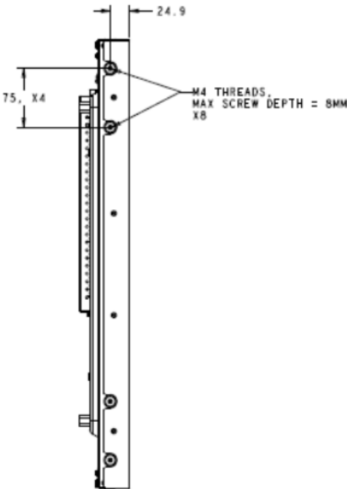
SIDE MOUNT VERITCAL (LEFT/RIGHT)
