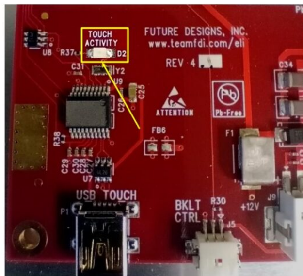
Figure 5. ELI121-CRW – Touch Activity LED
