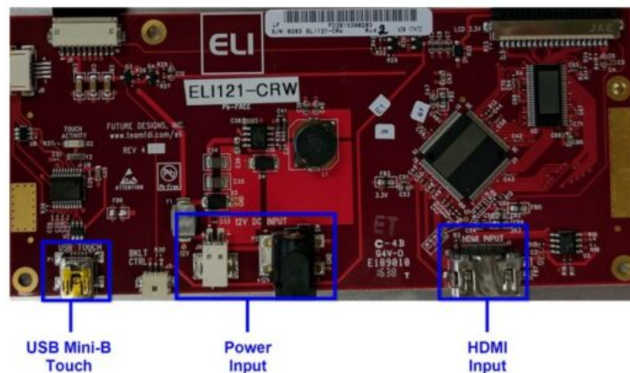
Figure 3. ELI121-CRW Connectors
