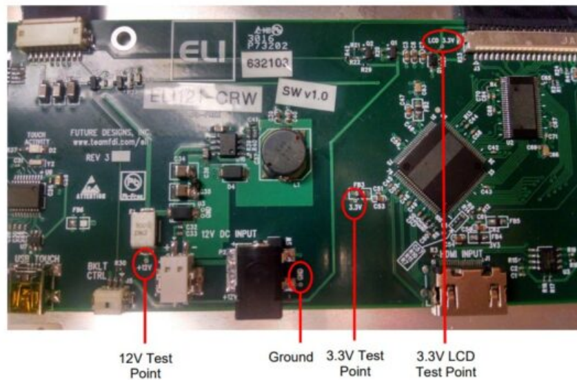
Figure 4. ELI121-CRW Power Test Points
