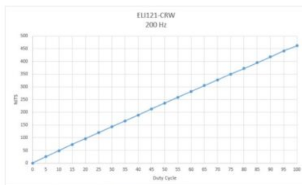
Figure 7. ELI121-CRW Backlight Curve in Nits
