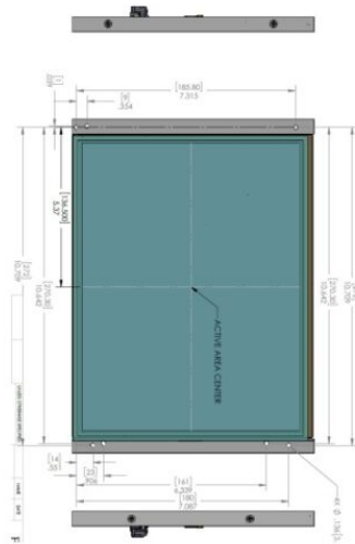
Figure 2. Dimensions of the ELI121-CRW including Mounting Brackets
