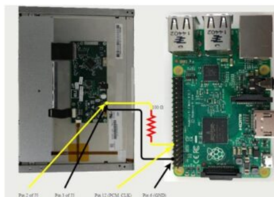
Figure 8 Raspberry Pi Signal and Ground
