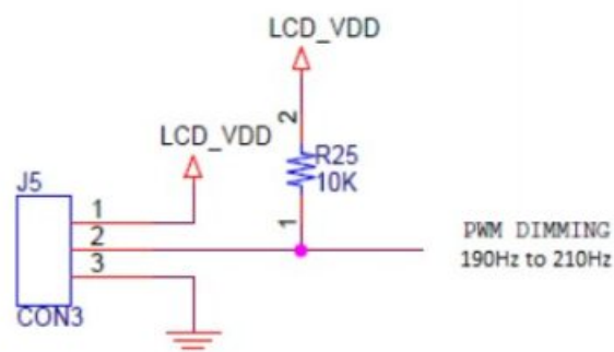
OPTIONAL PROCESSOR PWM BACKLIGHT CONTROL
