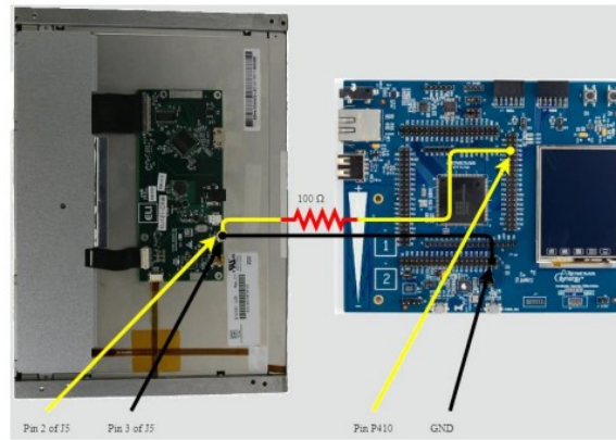
Figure 9. Renesas Synergy S7G2 Signal and Ground
