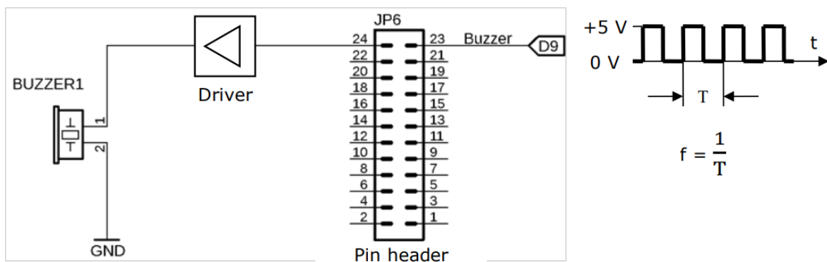
Figure 9: The wiring of Buzzer1
