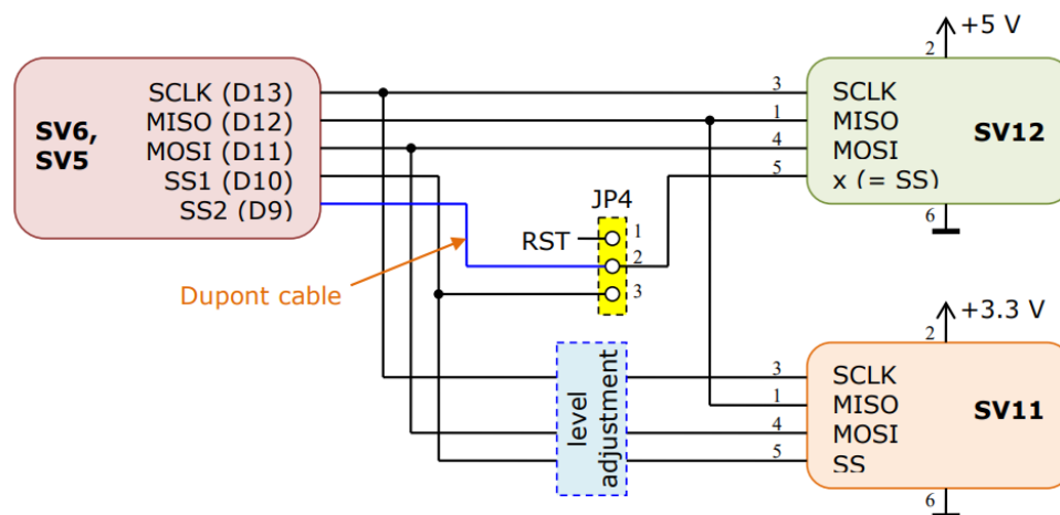
Figure 19: Simultaneous connection of two SPI modules to the MCCAB Training Board In this case, both SPI interfaces SV11 and SV12 may be connected to external SPI slaves at the same time, because both SV11 and SV12 use different SS lines now: LOW level at GPIO D10 activates the SPI module at SV11 and LOW level at GPIO D9 activates the SPI module at SV12 (see Figure 19).
