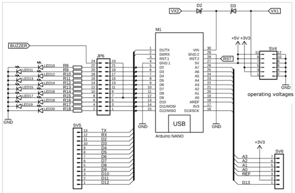
Figure 4: The wiring of the microcontroller module Arduino® NANO on the MCCAB Training Board The most important data of the microcontroller module Arduino® NANO:
