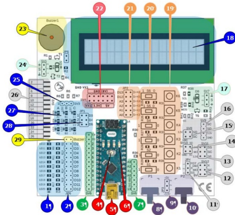
Figure 1: The MCCAB Training Board, Rev. 3.3
