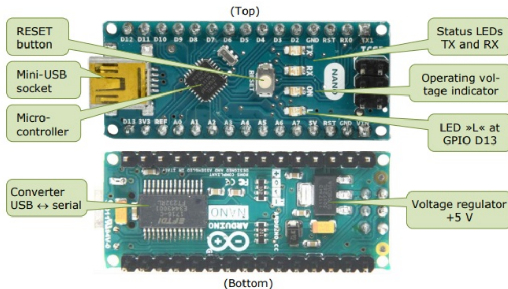
Figure 2: Microcontroller module Arduino® NANO (Source: www.arduino.cc )
