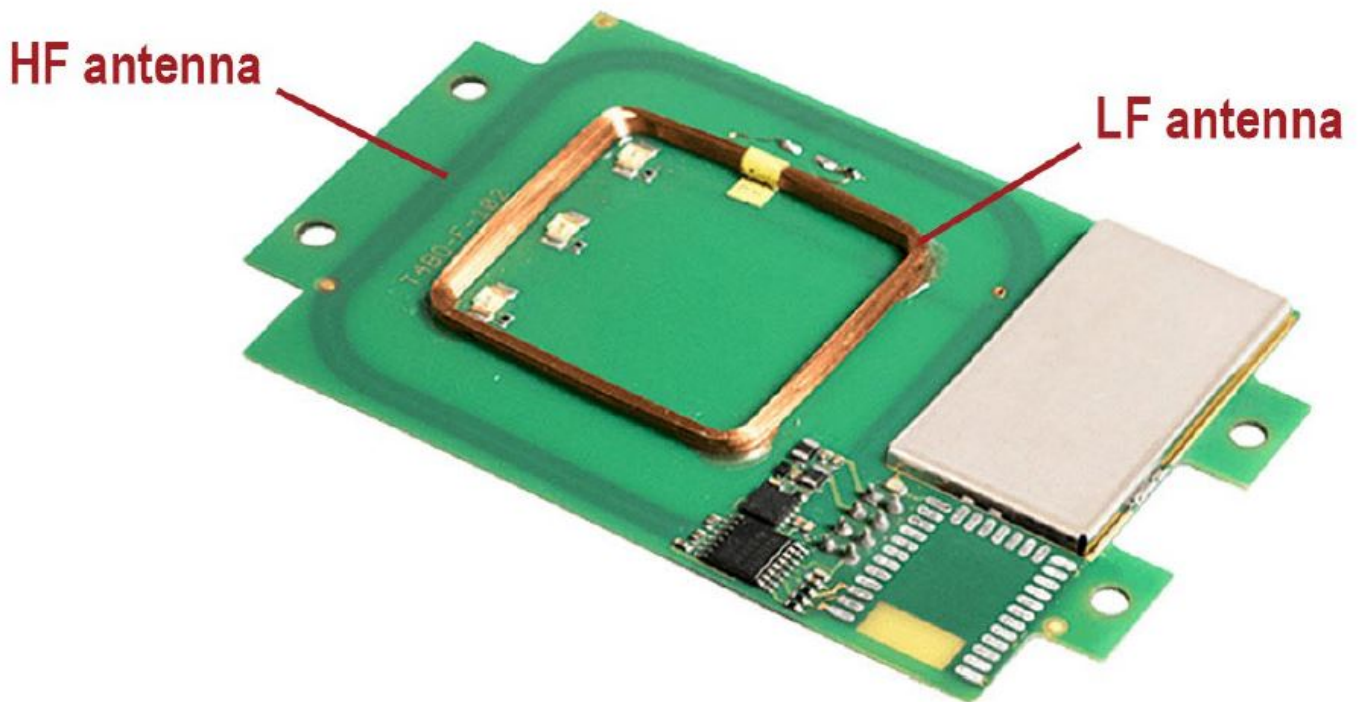
PCB contained in TWN4 MultiTech 2 LF HF
