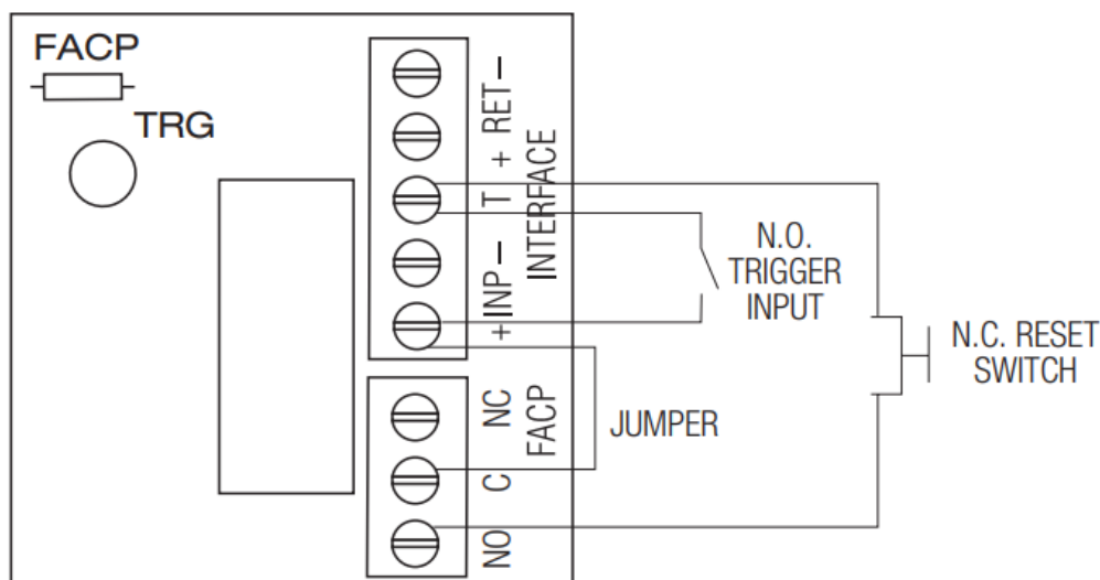
Fig. 9 Normally Closed: Non-Latching FACP trigger input:
