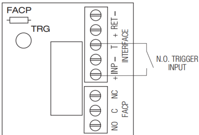
Fig. 7 Normally Open: Non-Latching FACP trigger input:
