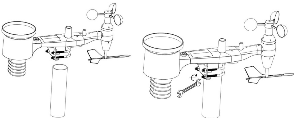
Figure 7: Sensor package mounting diagram
