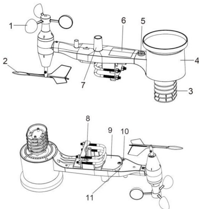
Figure 1: Sensor assembly components
