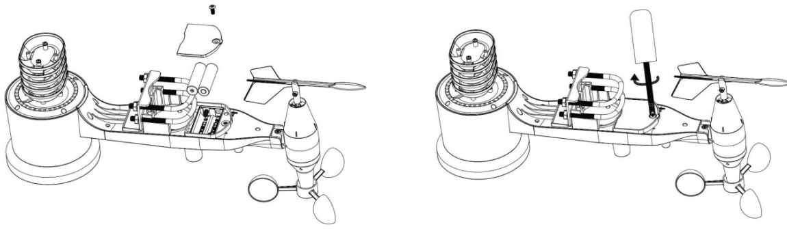
Figure 6: Battery installation diagram
