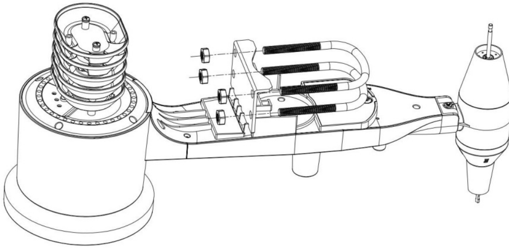
Figure 2: U-Bolt installation
