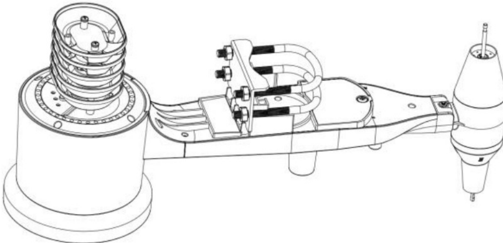
Figure 3: U-Bolts and nuts installed
