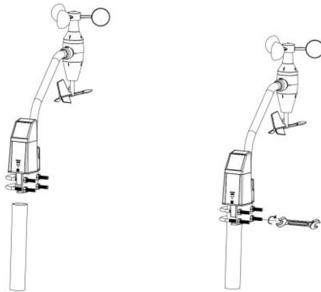
Figure 7: Sensor package mounting diagram
