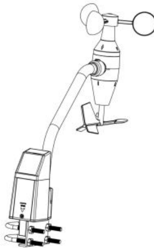
Figure 3: U-Bolts and nuts installed
