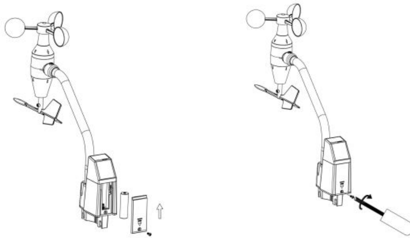
Figure 6: Battery installation diagram
