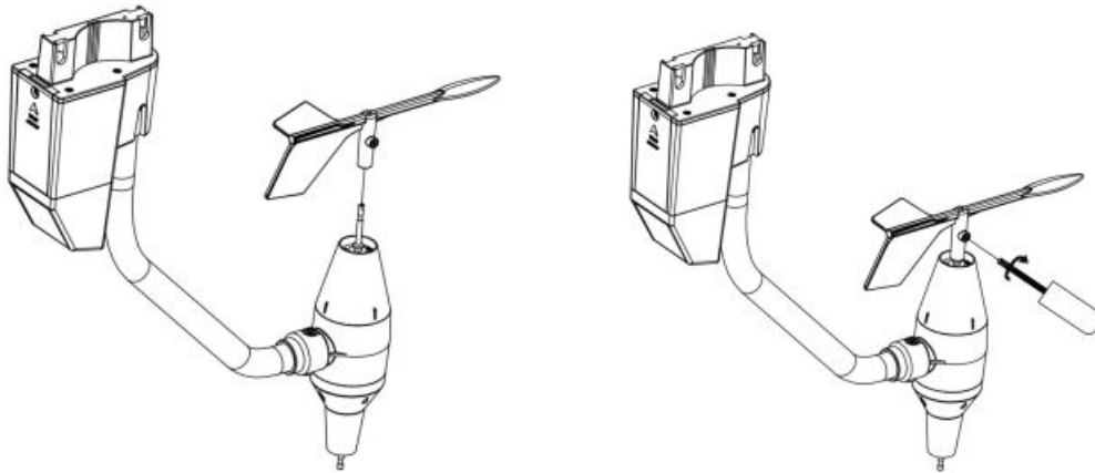
Figure 4: Wind vane installation diagram
