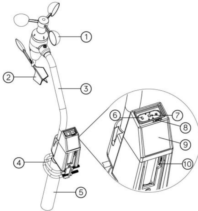
Figure 1: Sensor assembly components
