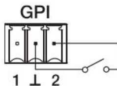
Figure 1: Connection example of GPI 2
