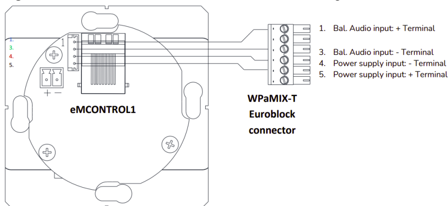
Figure 1: eMCONTROL1 + WPaMIX-T connection diagram
