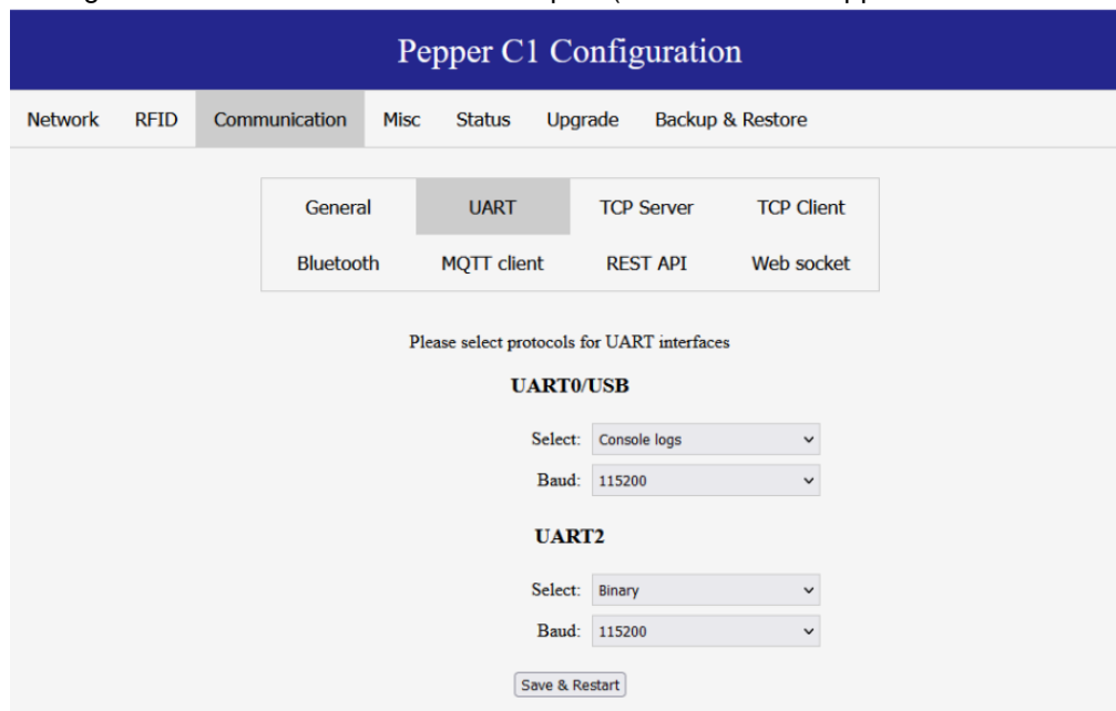
Figure 3-2. Console logs on the UART0/USB
