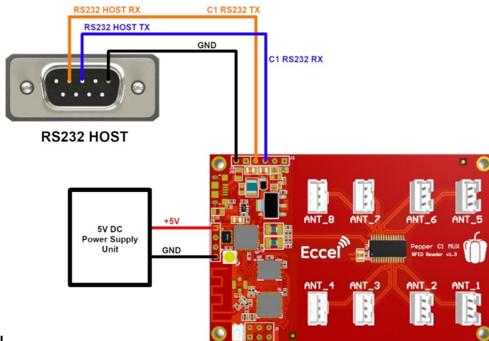
Figure 3-4. Pepper C1 MUX RS232 – typical connection with the RS232 host device
