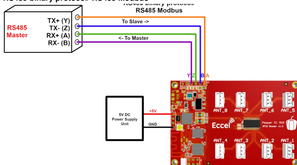
Figure 3-5. Pepper C1 RS485 – full duplex connection example
