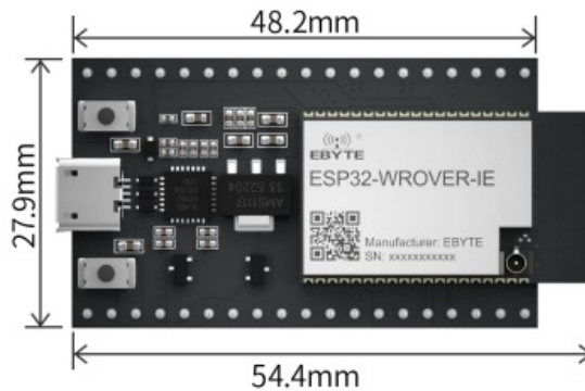
ESP32-WROVER-IE
