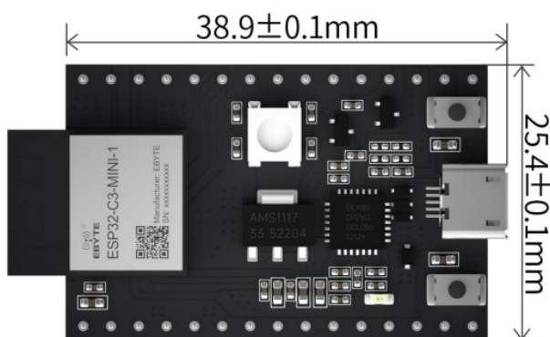
ESP32-C3-MINI-1-TB
