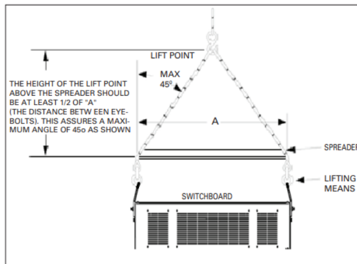
Figure 4. Top lifting with spreader
