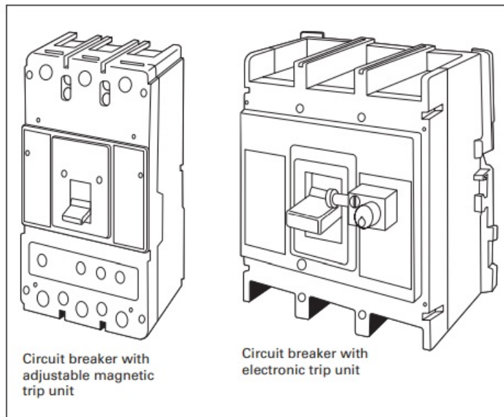
Figure 16. Circuit breakers
