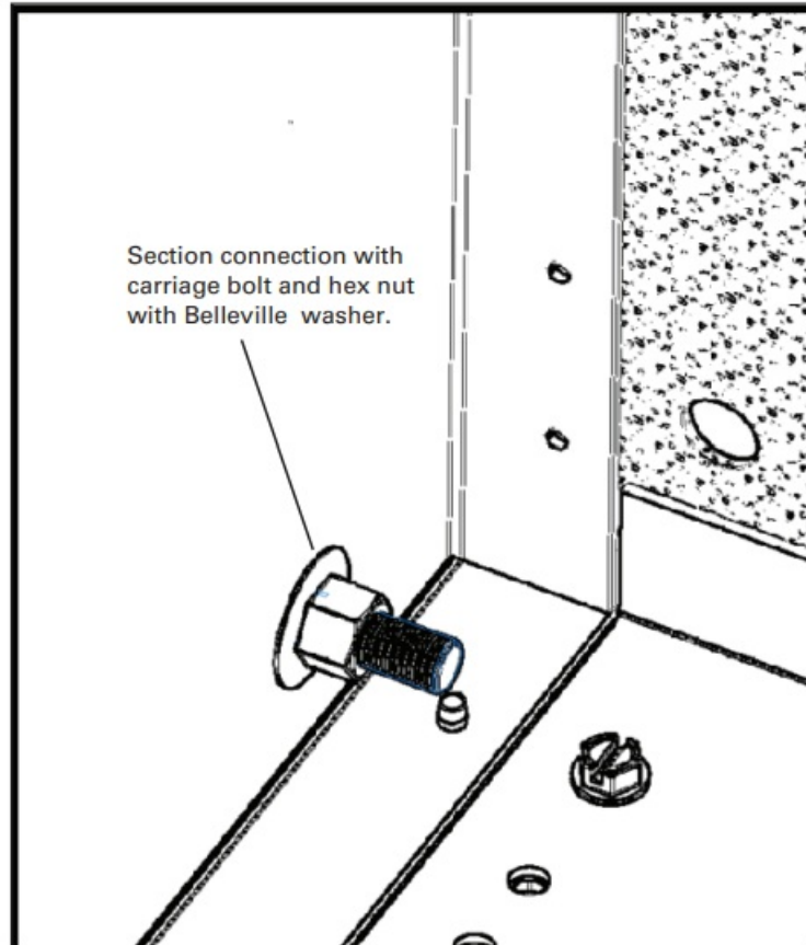
Figure 11. Switchboard section connection
