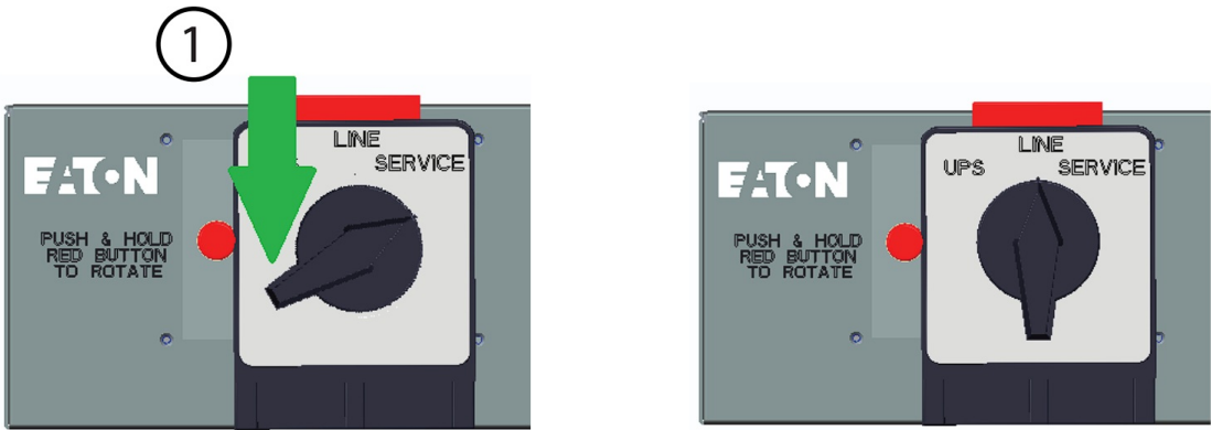
Figure 18. From SERVICE to LINE
