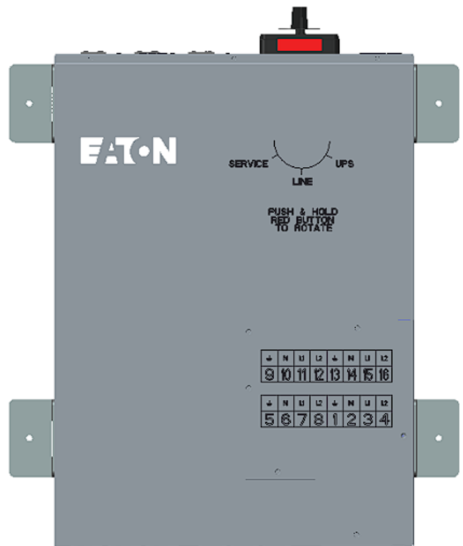
Figure 8. BPM with Wallmount Brackets
