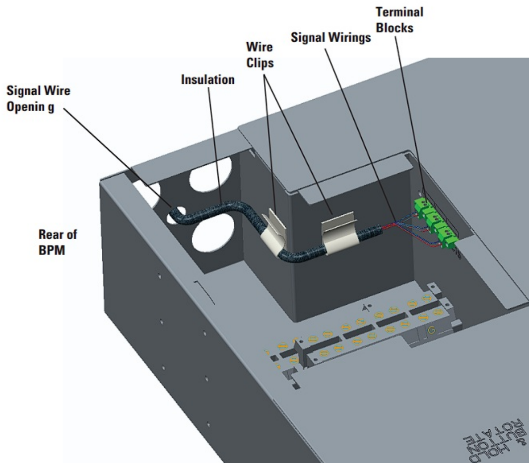
Figure 10. Signal Wire Routing
