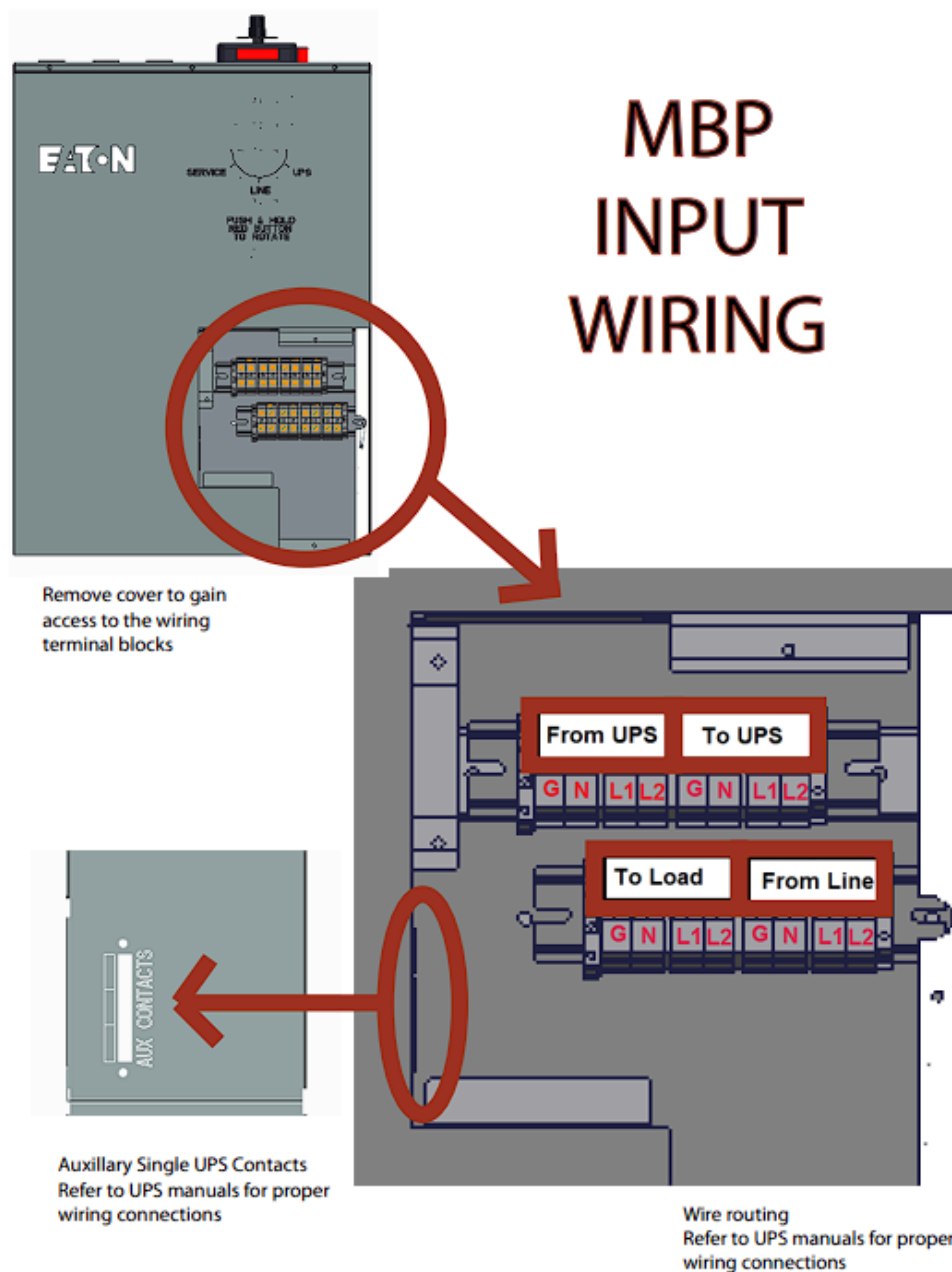
Figure 9. BPM Hardwired Overview
