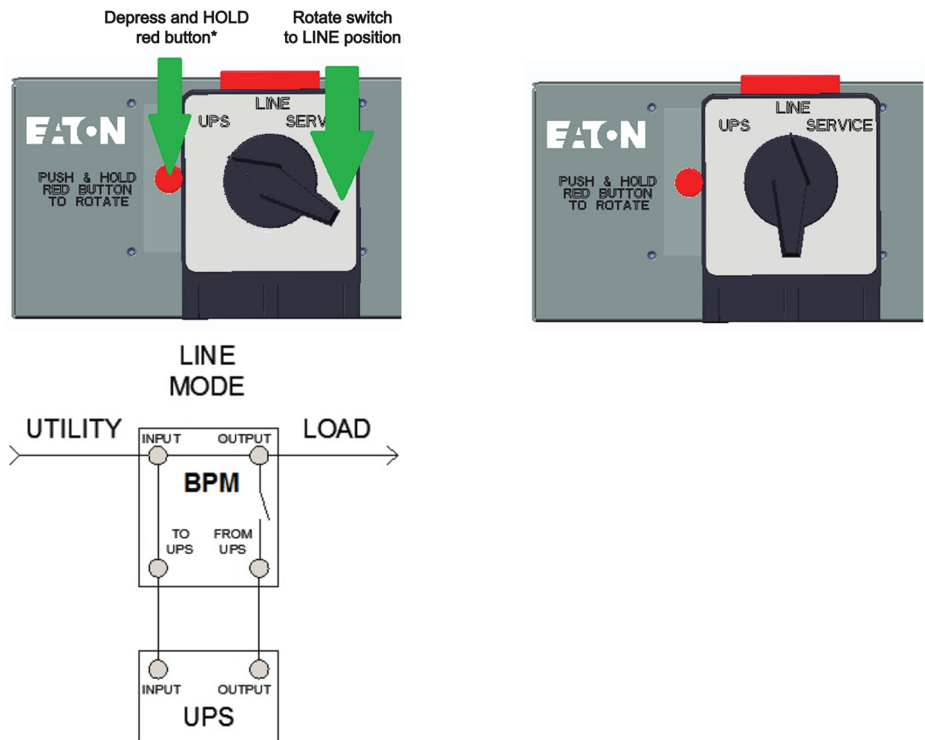
Figure 15. From UPS to LINE
