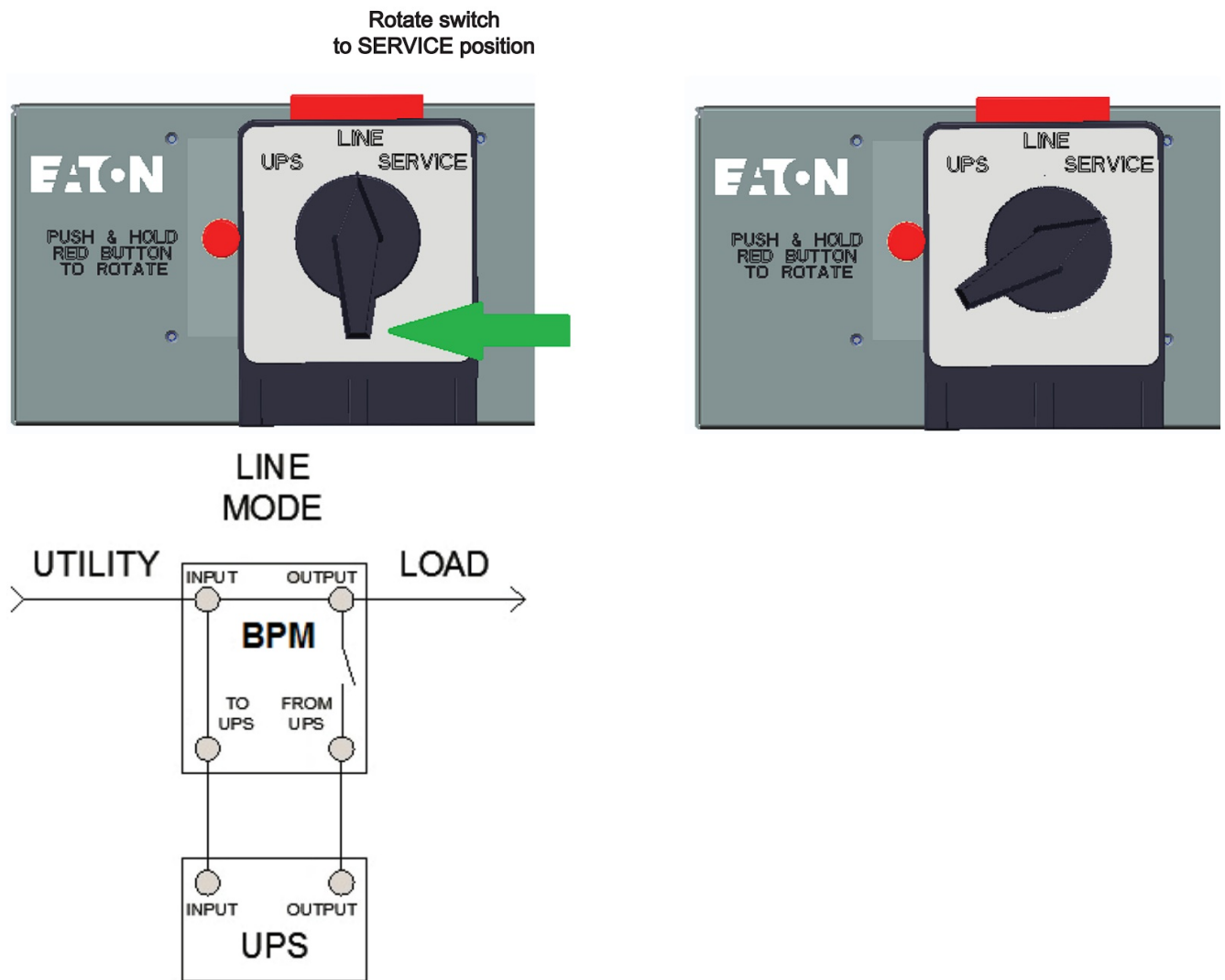
Figure 16. From LINE to SERVICE
