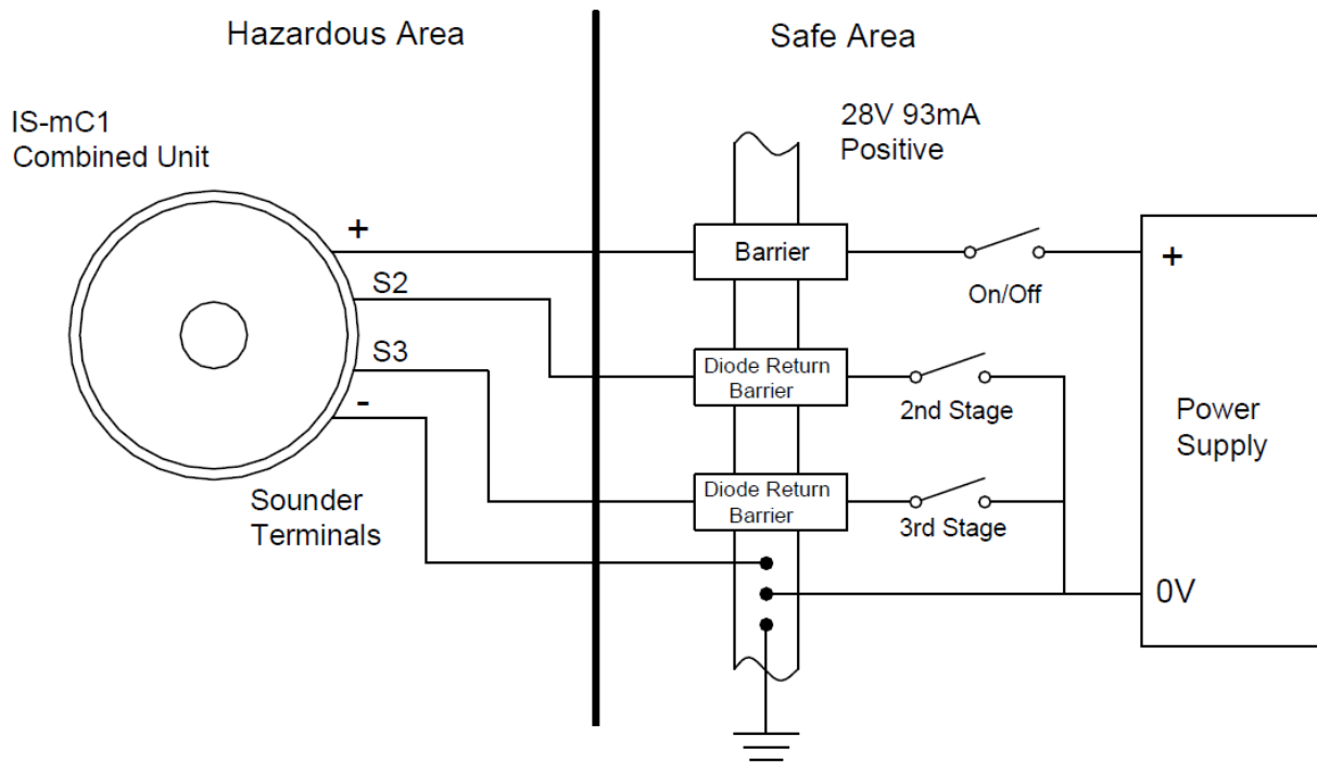
Fig 6: Sounder multi stage alarm using Zener barriers.
