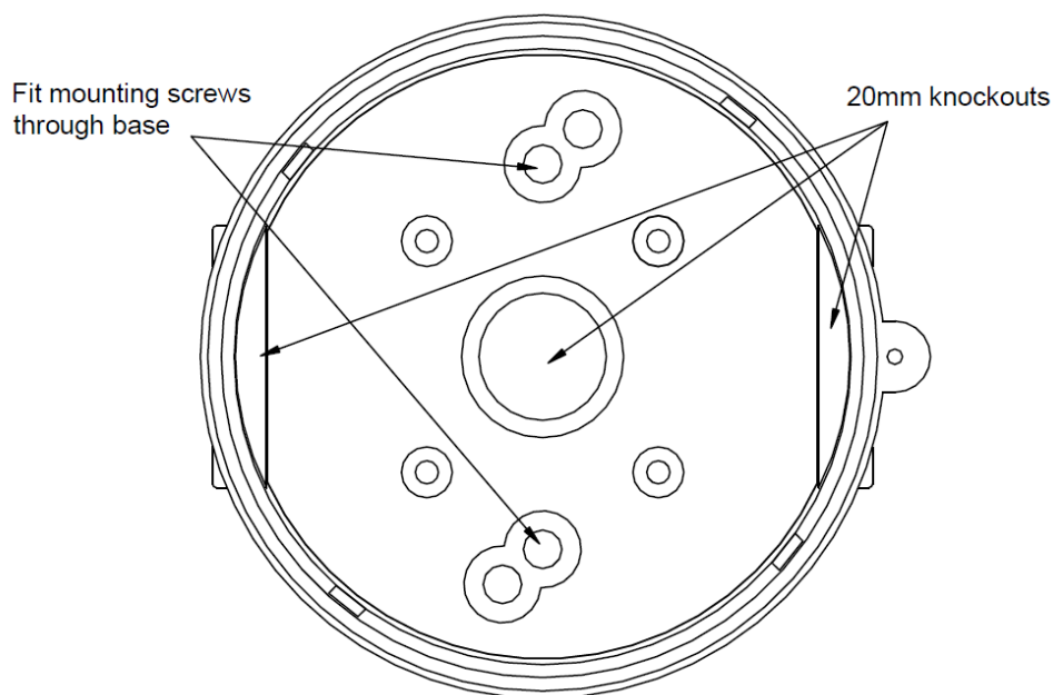
Fig 3: Mounting Combined Unit Base.
