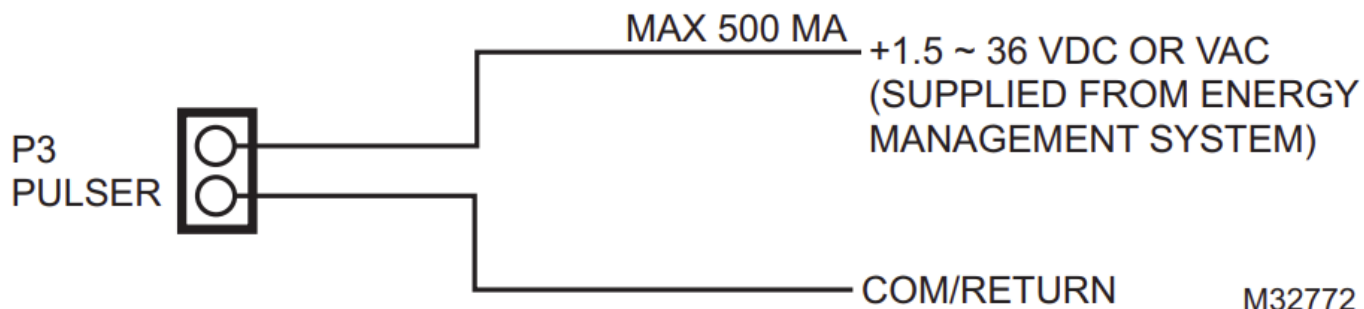
Fig. 1. Pulser Features
