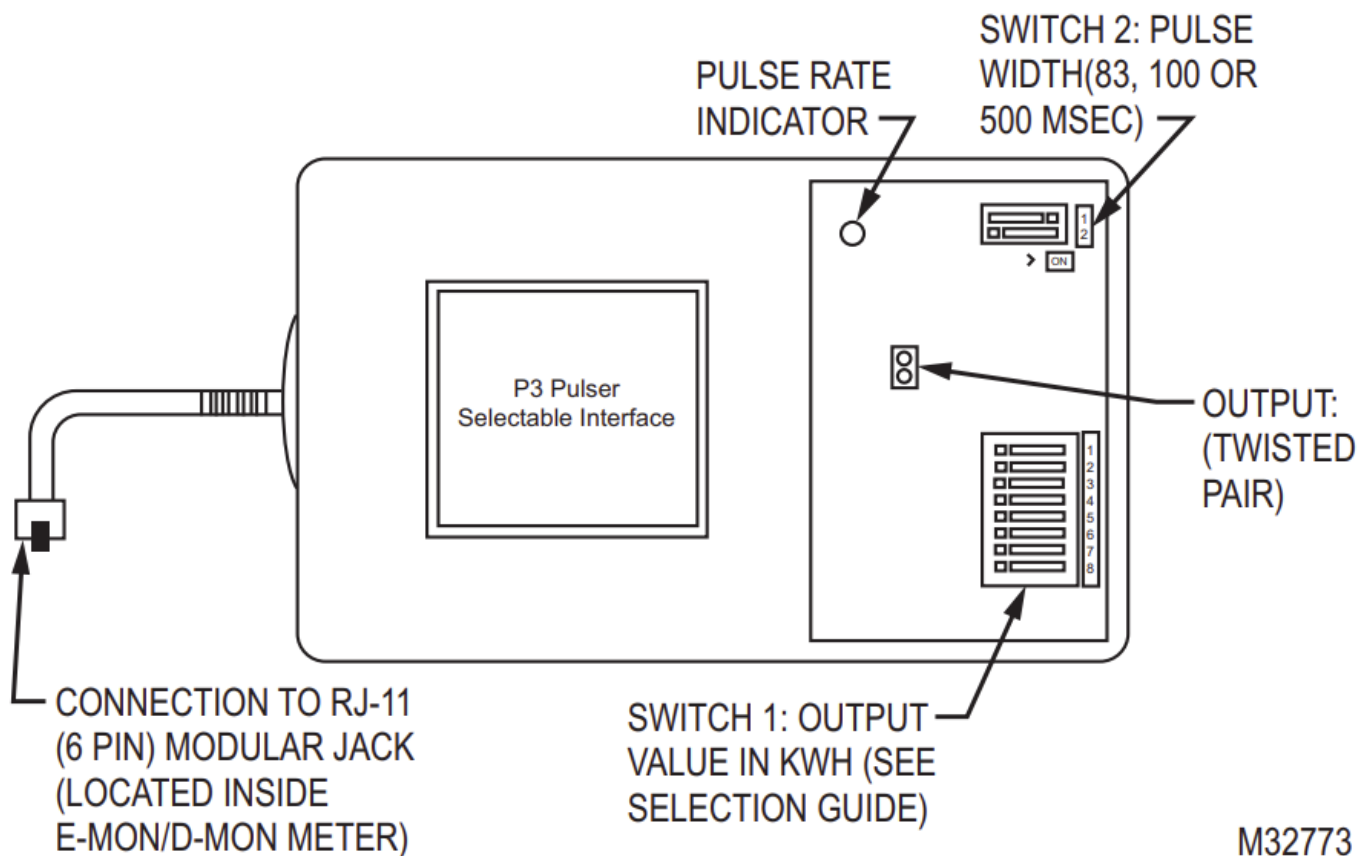
Fig. 1. Pulser Features
