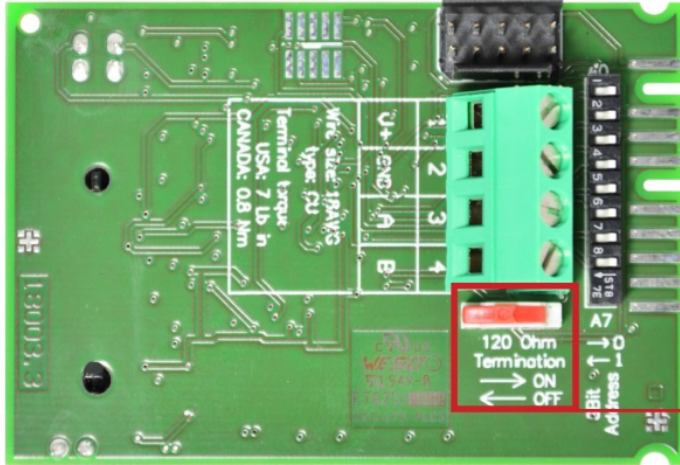
Bus termination resistor 120 \Omega (ON-OFF slide switch)
