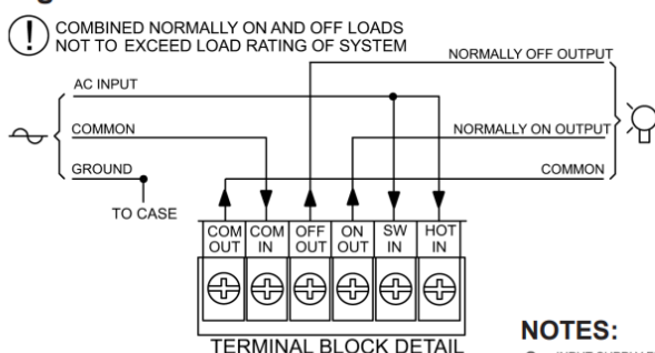
Diagram 3. NORMALLY ON & OFF LOADS
