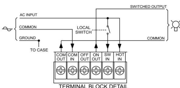
Diagram 4. SWITCHED LOADS
