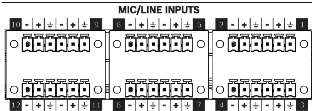
Figure 5.1: Analog input connections
