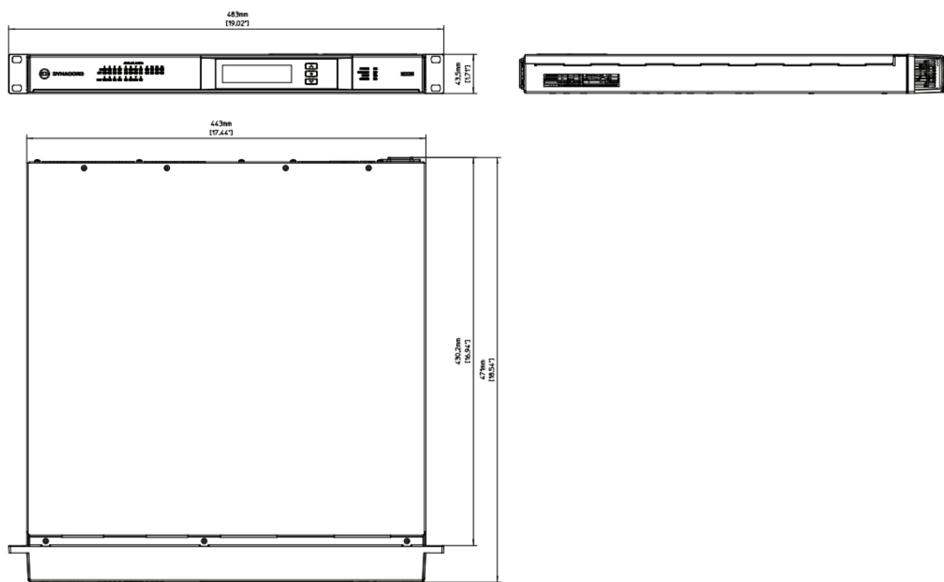
Figure 7.1: Dimensions: MXE5
