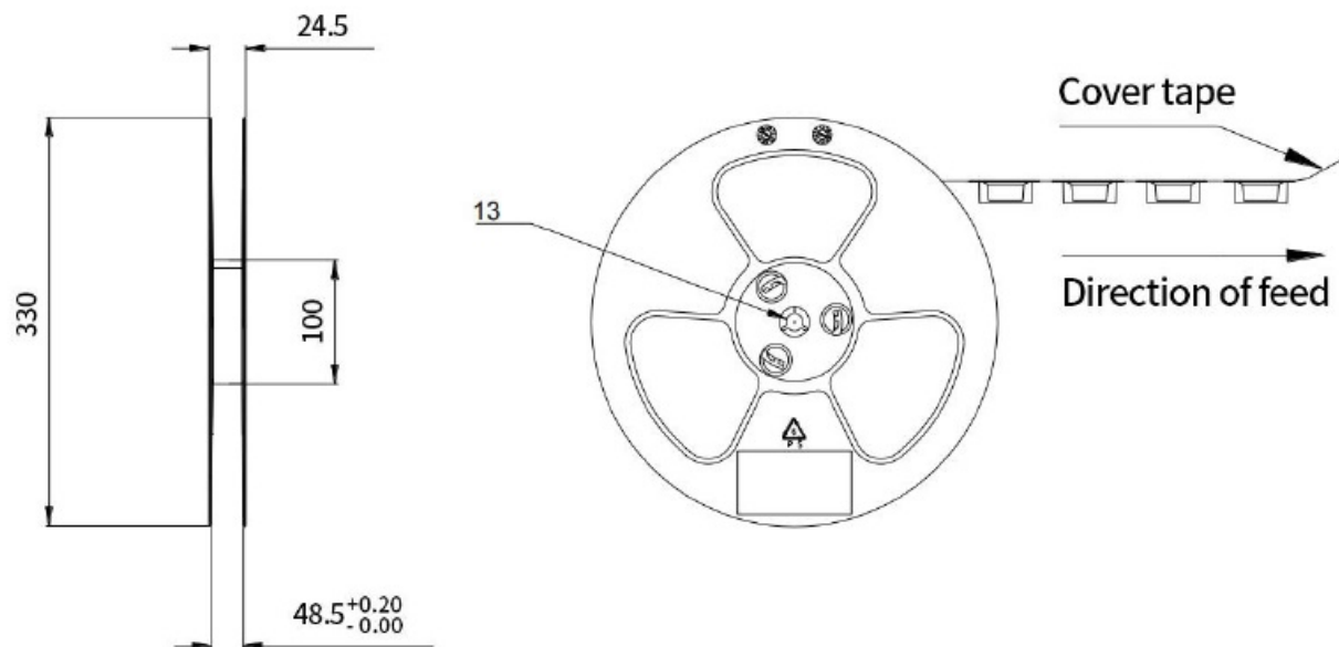
Figure 24 : Reel dimensions (unit: mm)
