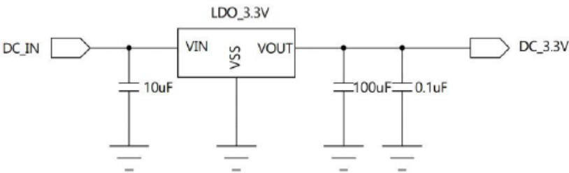
Figure 4 : Power supply reference circuit
