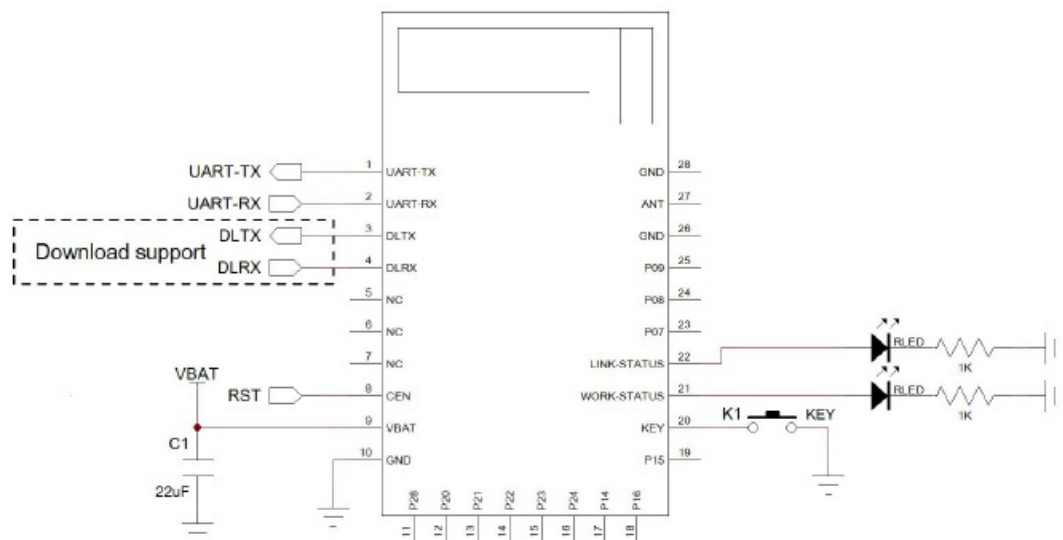
Figure 16 : Typical application circuit
