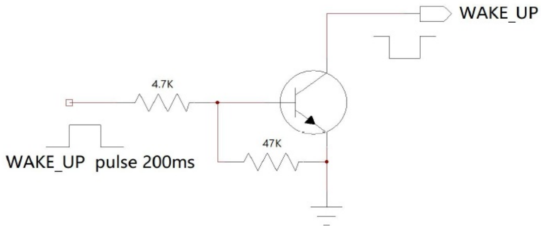
Figure 7 : KEY reference circuit
