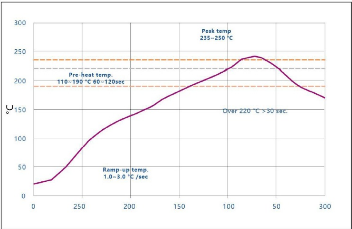
Figure 22 : Recommended reflow temperature profile
