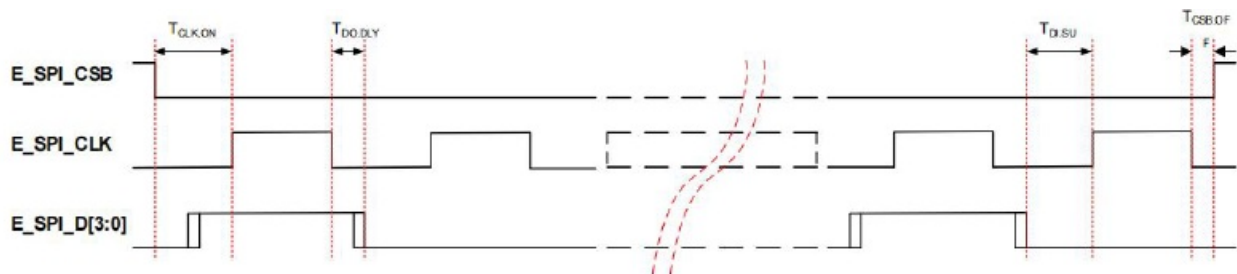
Figure 11 : SPI communication timing diagram
