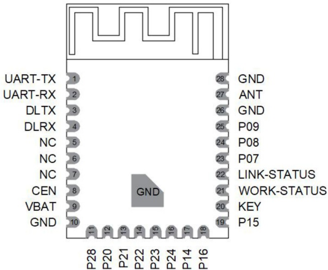
Figure 2 : Module pin definition
