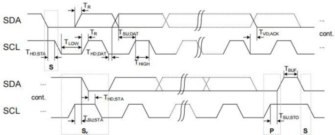
Figure 9 : I2C communication timing diagram
