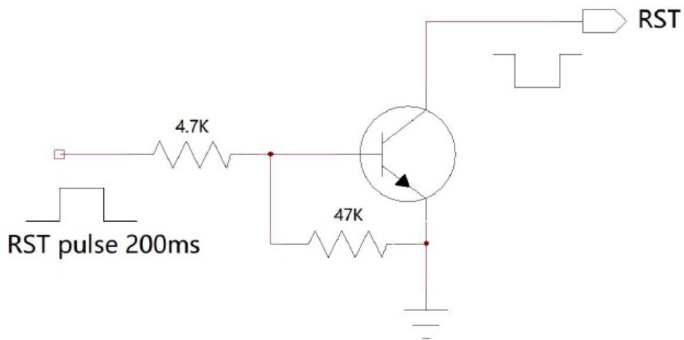
Figure 5 : Reset reference circuit
