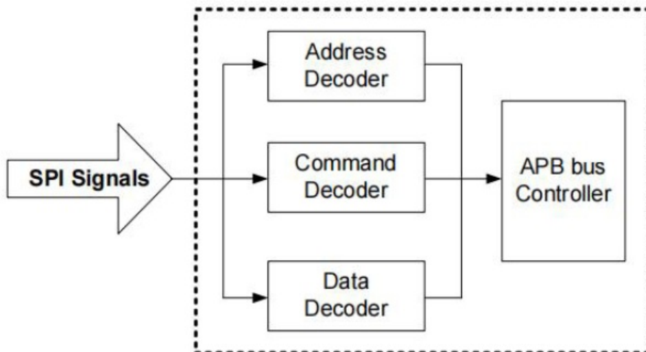
Figure 12 : SPI Slave Block Diagram
