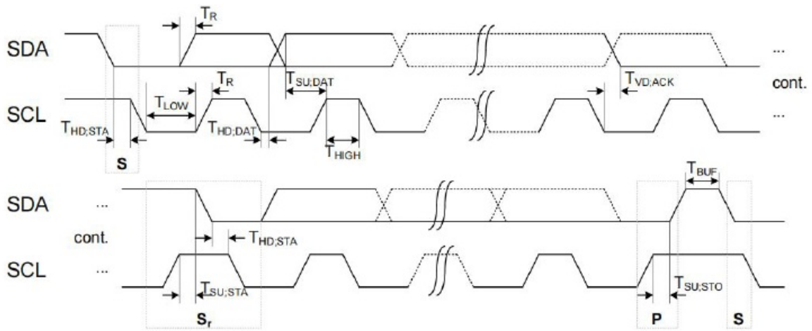
Figure 9 : I2C communication timing diagram
