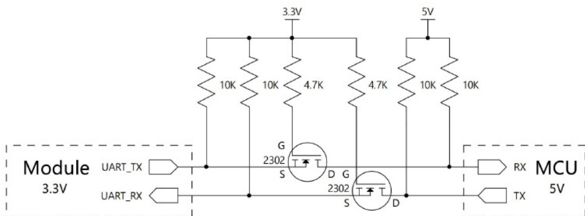
Figure 17 : Serial port level conversion reference circuit
