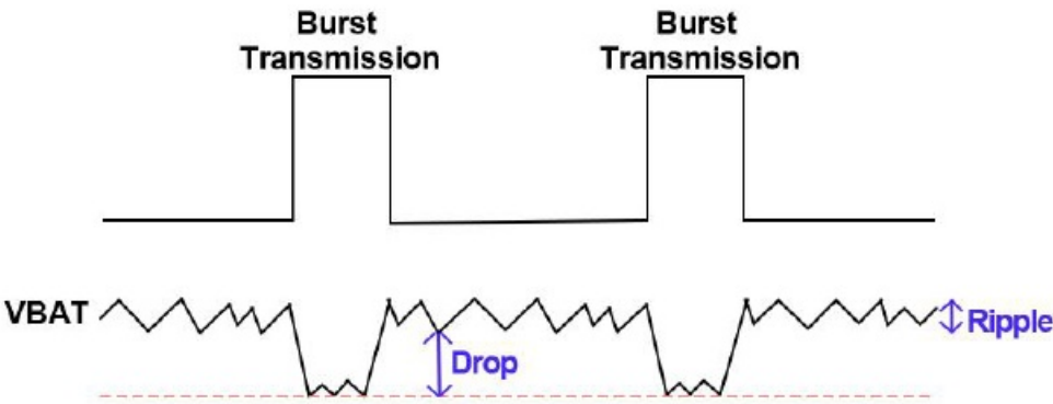
Figure 3 : Burst transmission power requirements
