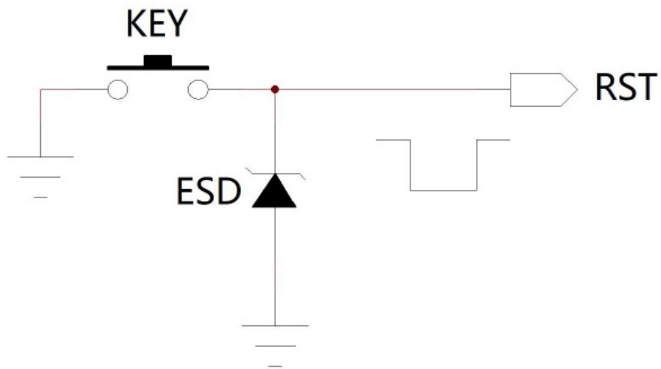
Figure 6 : Push button reset reference circuit
