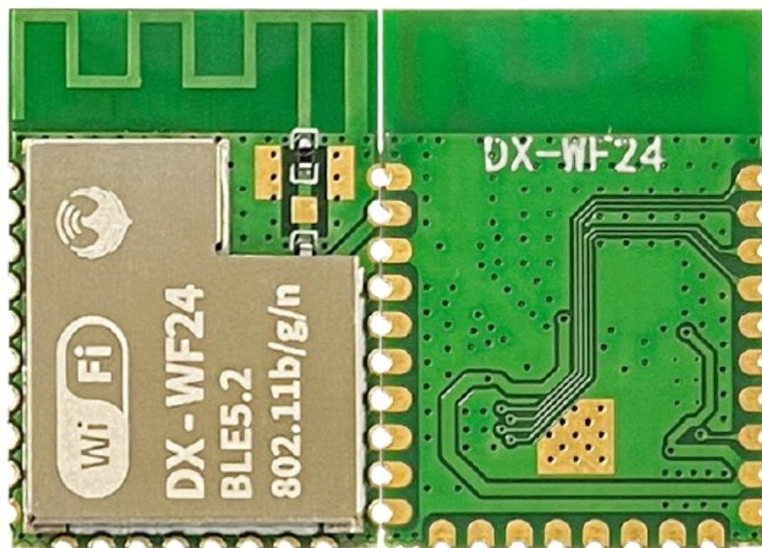
Figure 20 : Module top and bottom views
