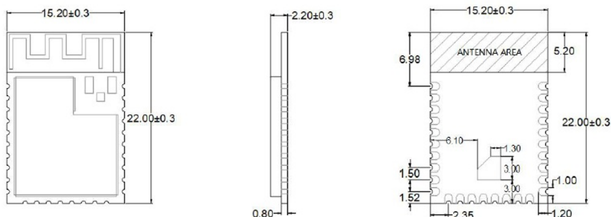
Figure 18 : Module top and side view dimensions
