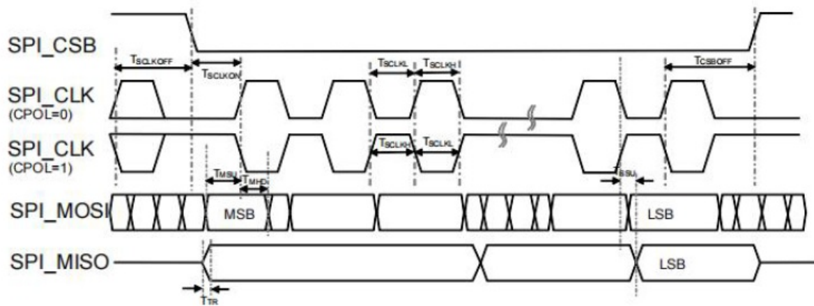
Figure 15 : SPI slave timing diagram
