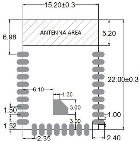
Figure 19 : Recommended package dimensions
