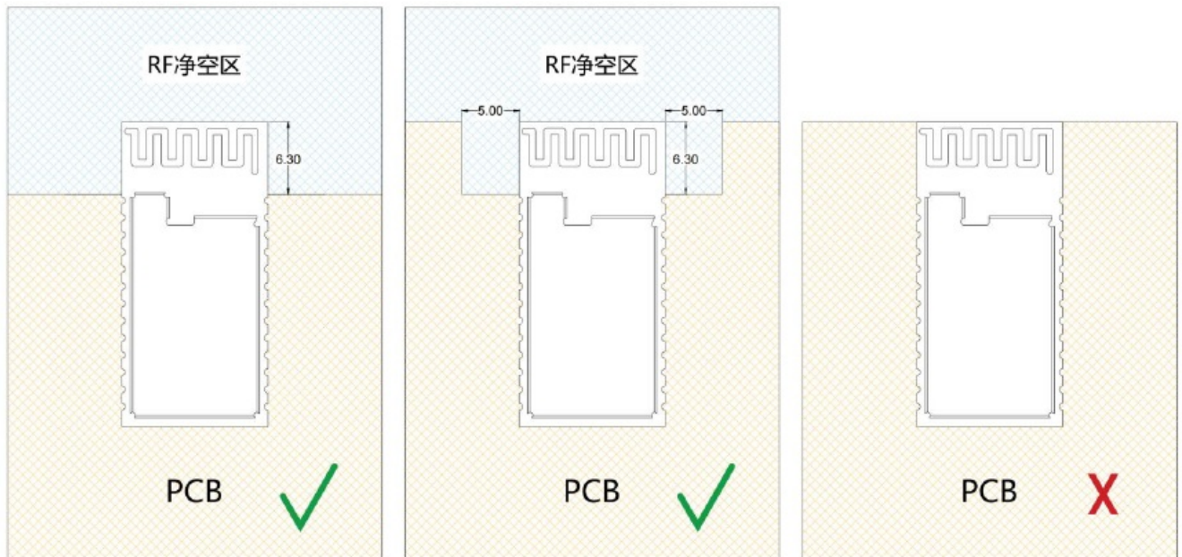
Figure 21 : Module placement reference position
