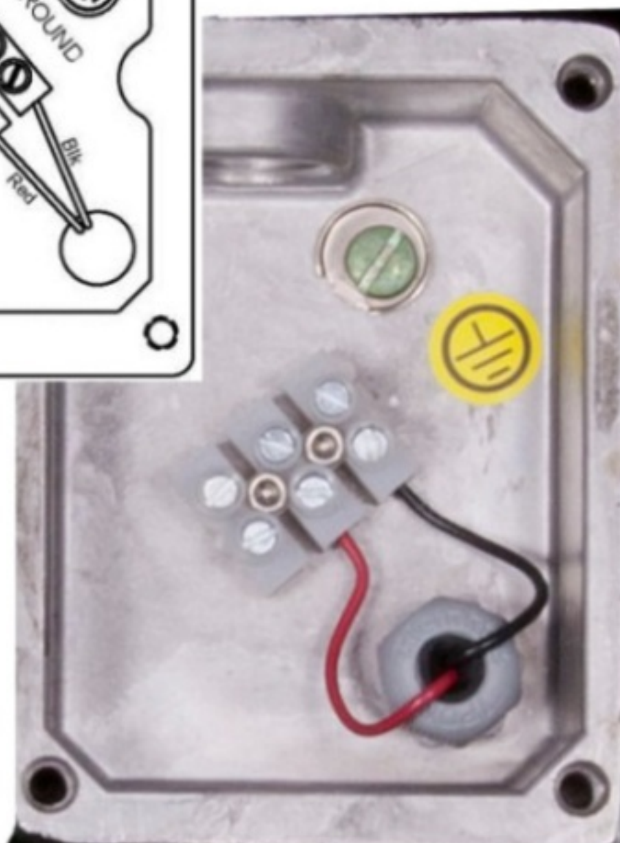
Figure 17: Transmitter Wiring with or without HART
