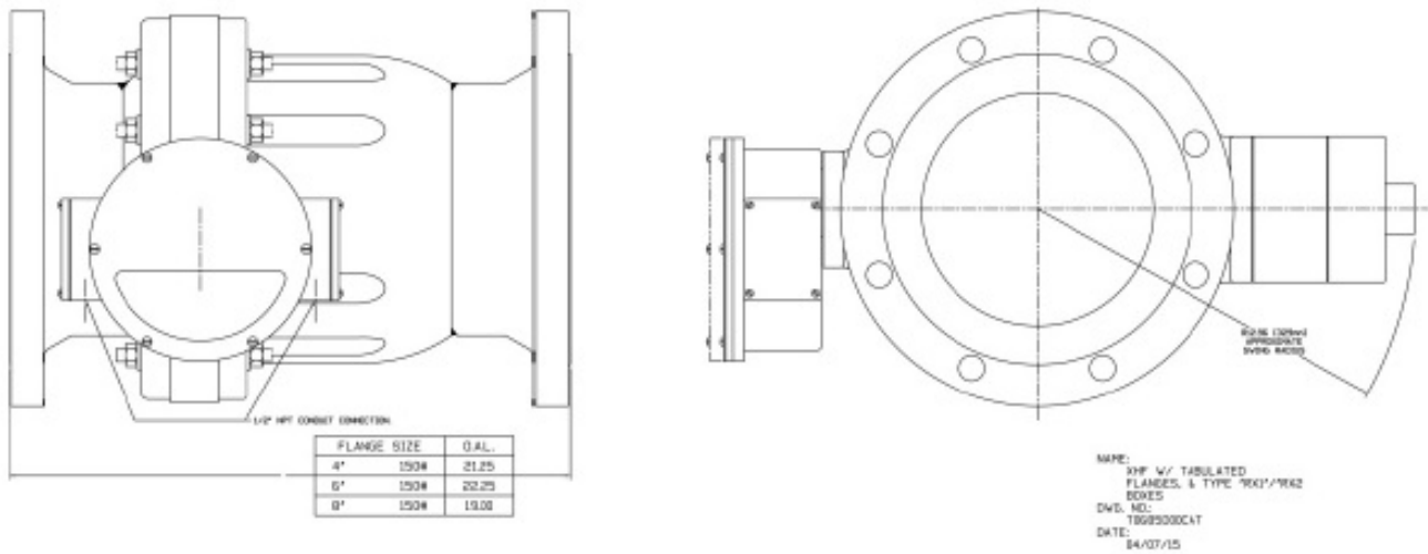
Figure 15: XHF Dimensions
