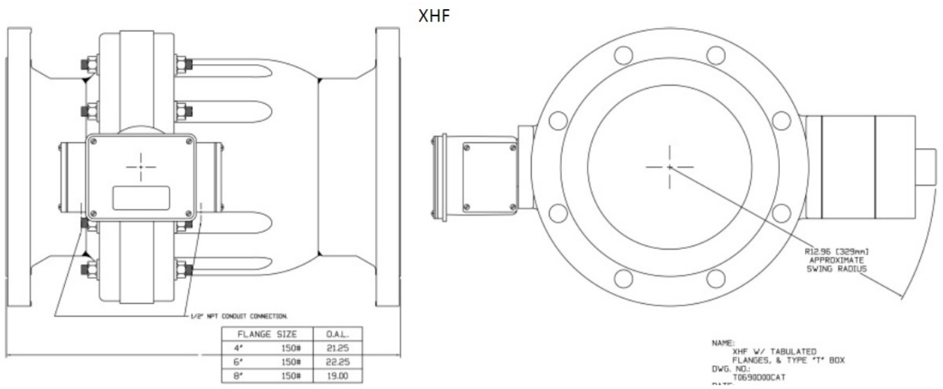
Figure 24: XHF dimensions
