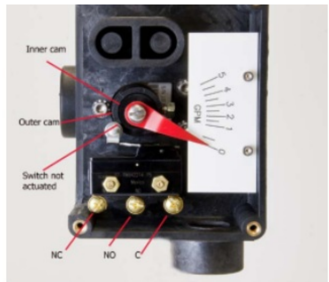
Figure 2: Device overview
