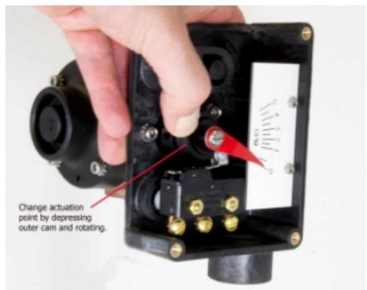
Figure 3: Cam adjustment
