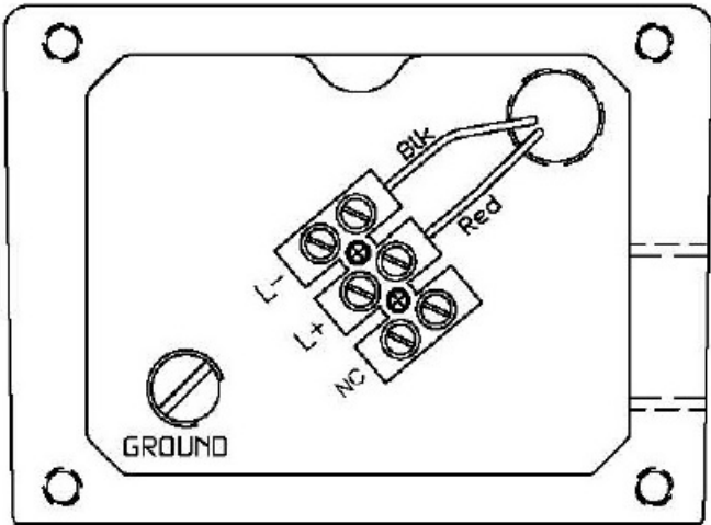
Figure 30: PCB Wiring
