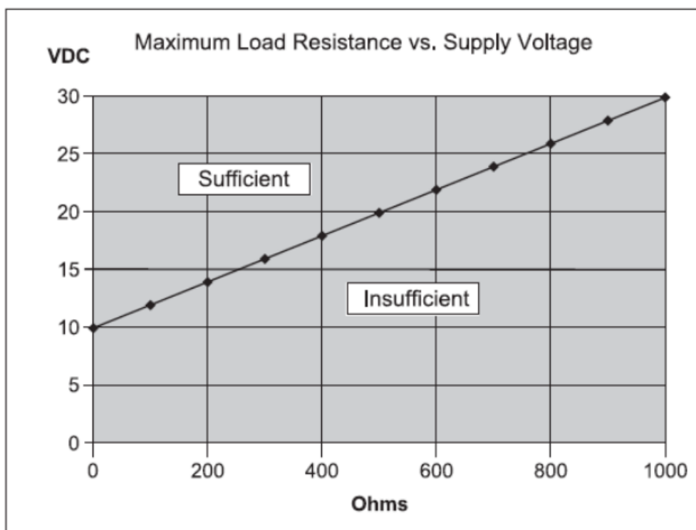
Figure 28: Maximum Load Resistance vs. Supply Voltage
