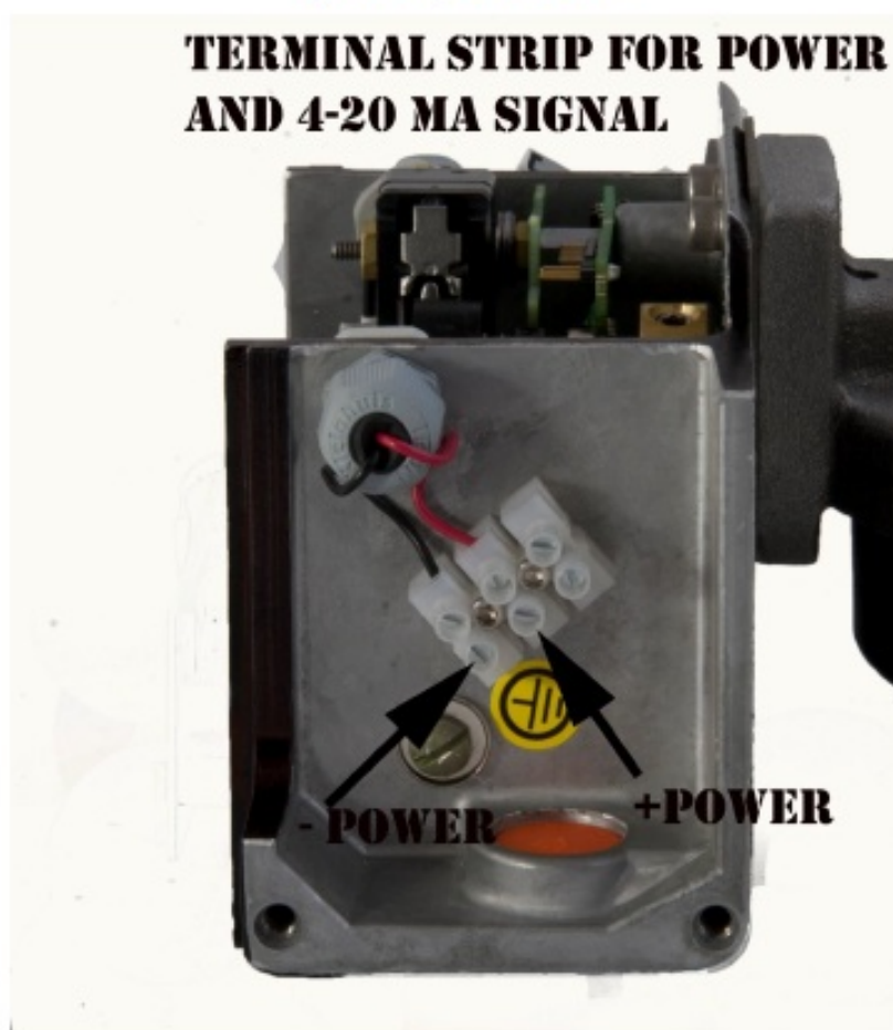
Figure 32: Terminal Strip for Power and 4-20 mA Signal
