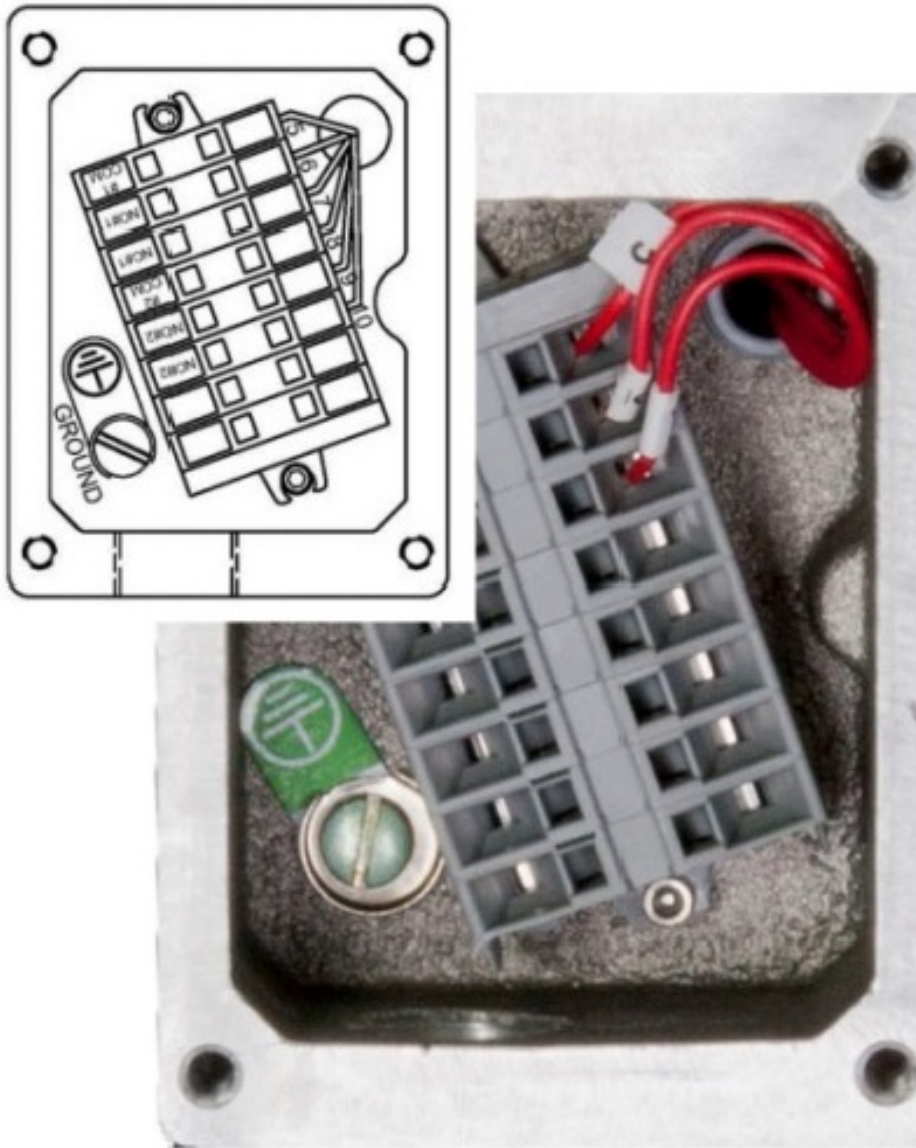
Figure 18: Mechanical (Optional) Switch Wiring
