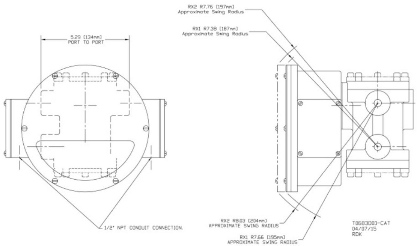
Figure 13: LL, LP, and LH Dimensions
