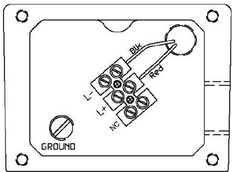
Figure 21: PCB Wiring
