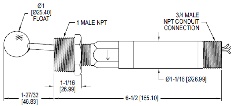
Round stainless steel float
