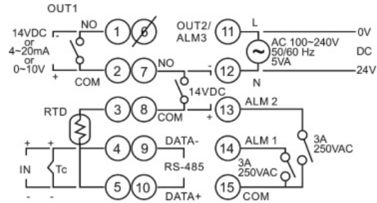
DC, No Event/CT Input
