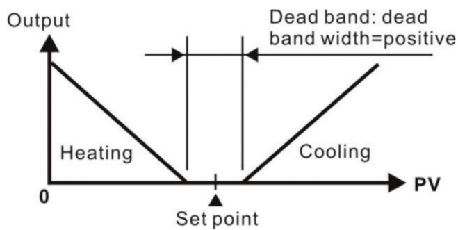
PID control Dead Band is positive.
