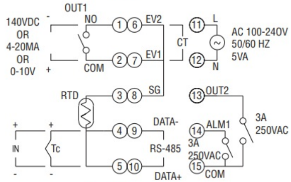
AC, Event / CT Input
