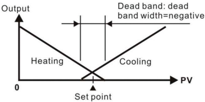
PID control, Dead Band is negative.
