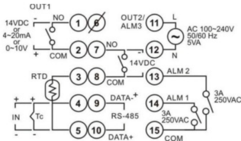
AC, No Event / CT Input
