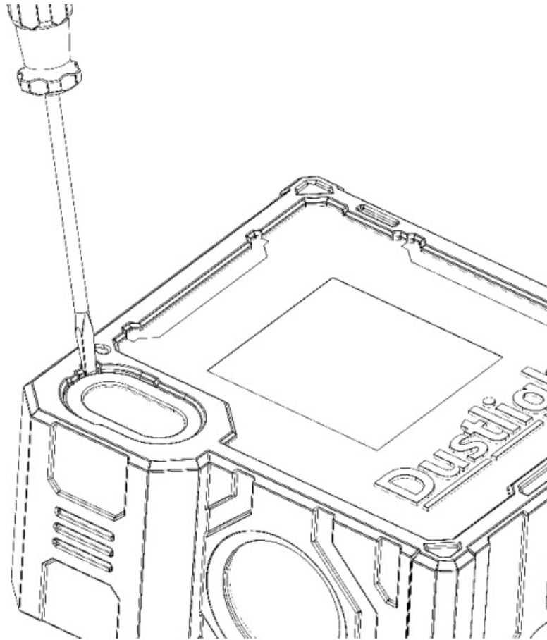
Illustration 1: Removing the protective grille on the air inlet
