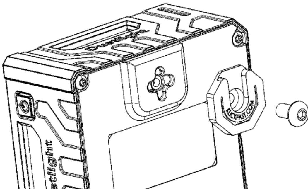
Illustration 5: Mounting the Klick-Fast connector
